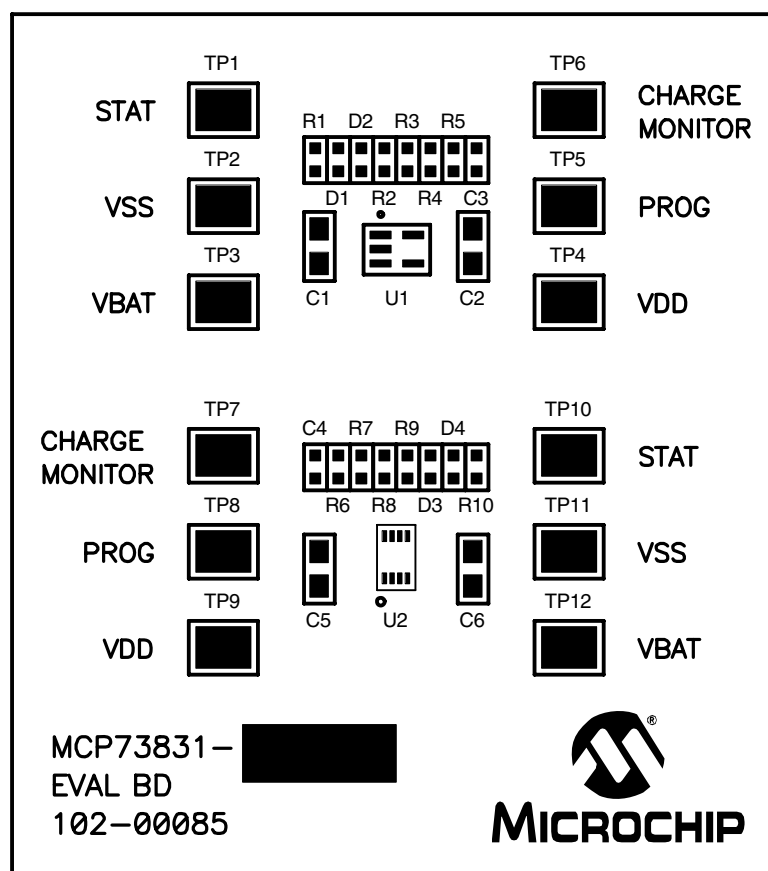
FIGURE A-3: Board - Top Overlay.
