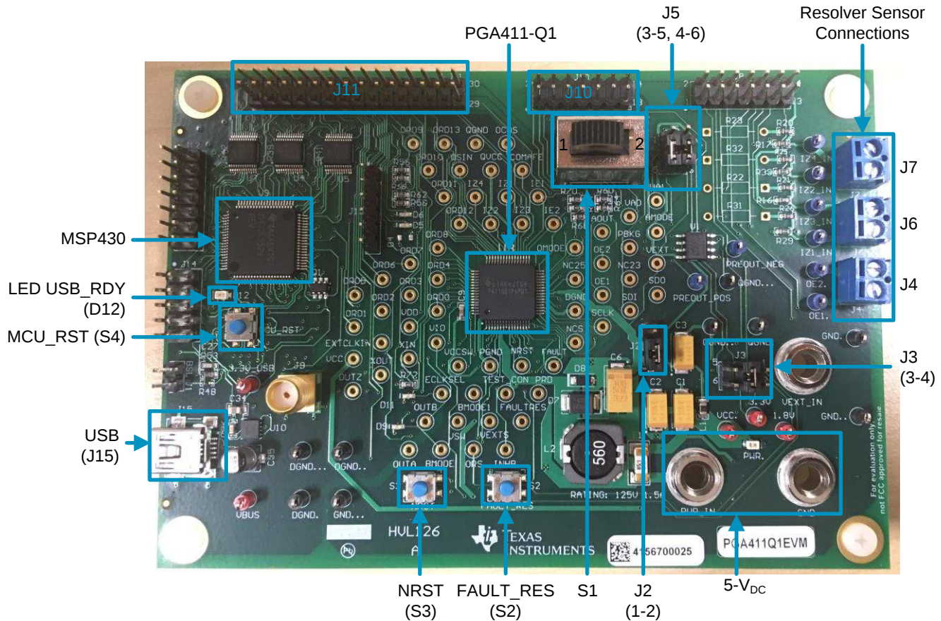
Figure 2. PGA411-Q1 EVM
