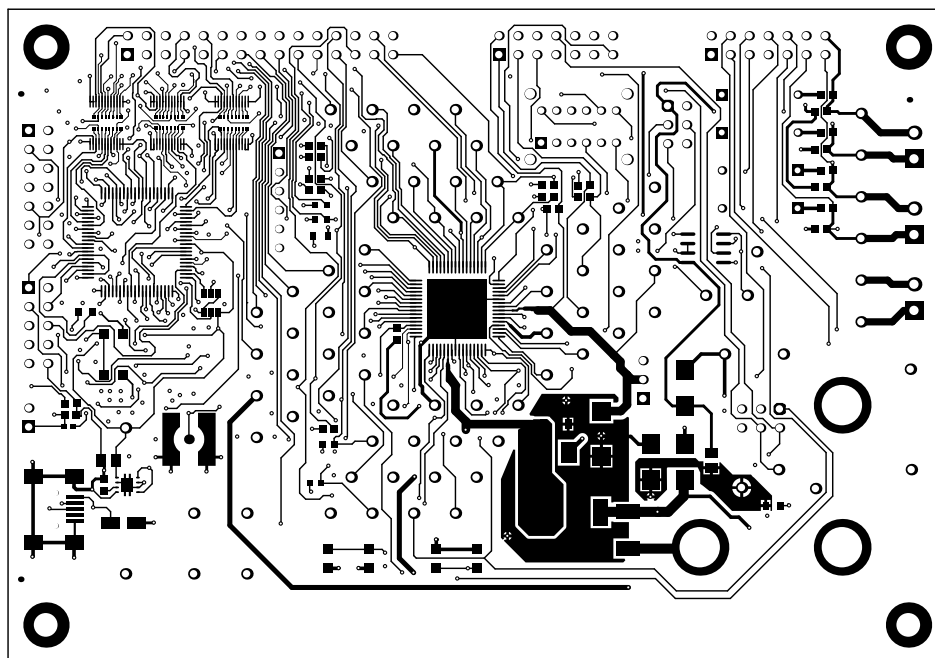
Figure 24. Top-Side Layout
