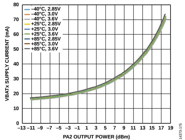
Figure 74. VBATx Supply Current vs. PA2 Output Power, Temperature, and V_{DD} with PA_COARSE = 10, PAOLDO_VOUT_CON = 15, RF Frequency = 915 MHz
