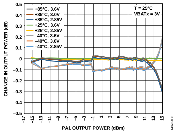
Figure 28. Change in PA1 Output Power vs. Temperature, and V_{DD} with PA_COARSE = 6, RF Frequency = 433 MHz
