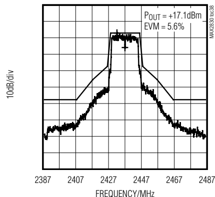
TRANSMIT EMISSION MASK
