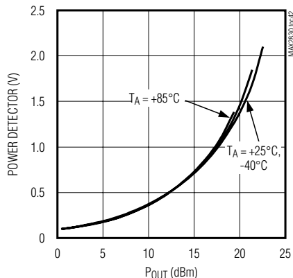
POWER DETECTOR OVER TEMPERATURE
