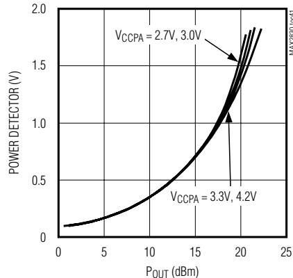
POWER DETECTOR OVER SUPPLY VOLTAGE
