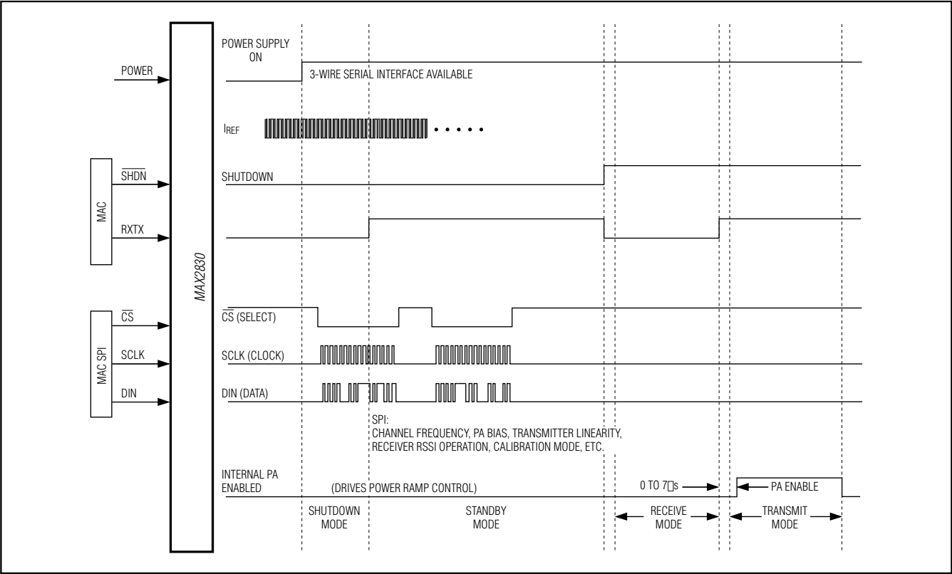
Figure 4. Timing Diagram
