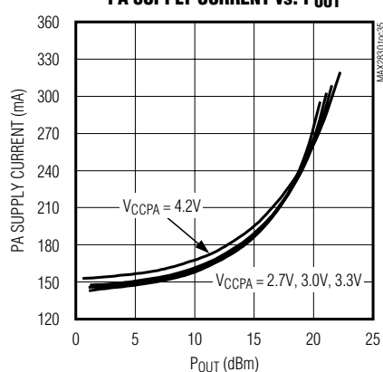
PA SUPPLY CURRENT vs. P_{OUT}
