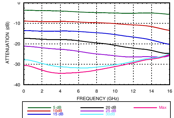
Relative Attenuation
