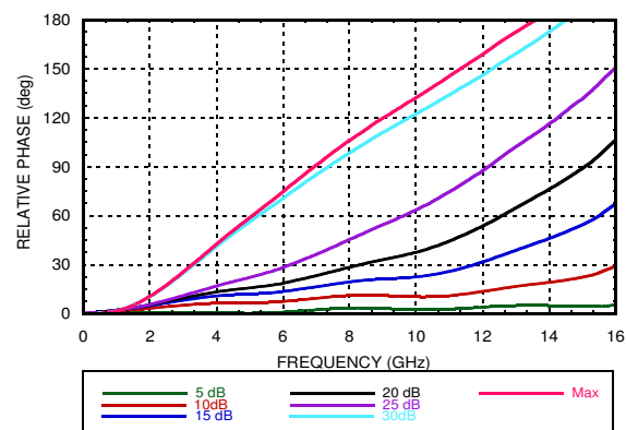
Relative Phase
