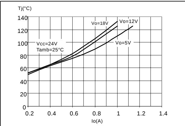
Figure 22. Junction temperature vs. output current ( V_{CC} = 24\text{ V} )
