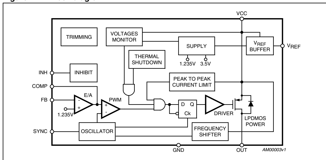
Figure 4. Block diagram
