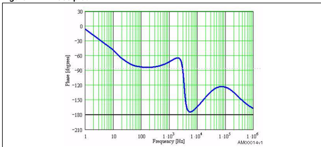
Figure 12. Phase plot
