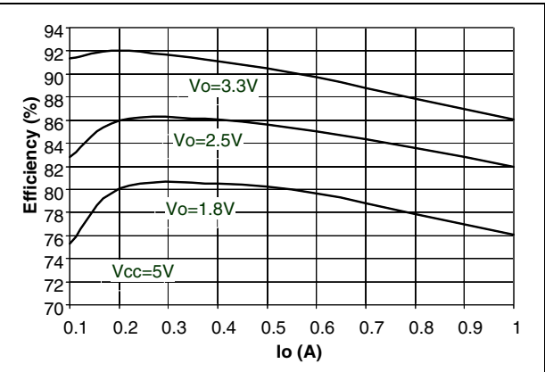
Figure 23. Efficiency vs. output current ( V_{CC} = 5\text{ V} )
