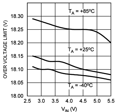
Over Voltage Limit vs V_{IN} ( V_{OUT} Falling)
