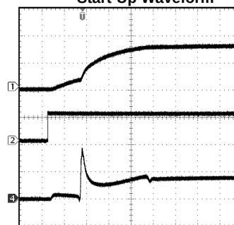
Start-Up Waveform
