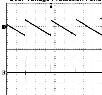
Over-Voltage Protection Function
