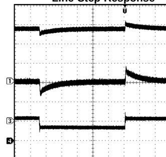
Line-Step Response
