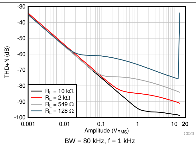
Figure 24. THD+N vs Output Amplitude
