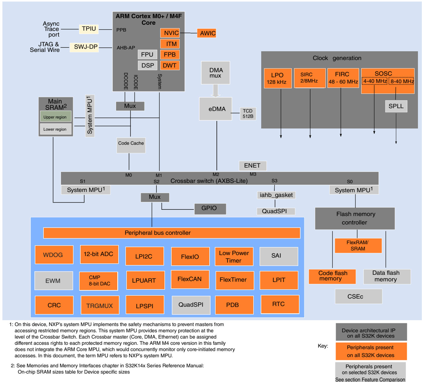
Figure 1. S32K1xx Product Series high-level architecture diagram
