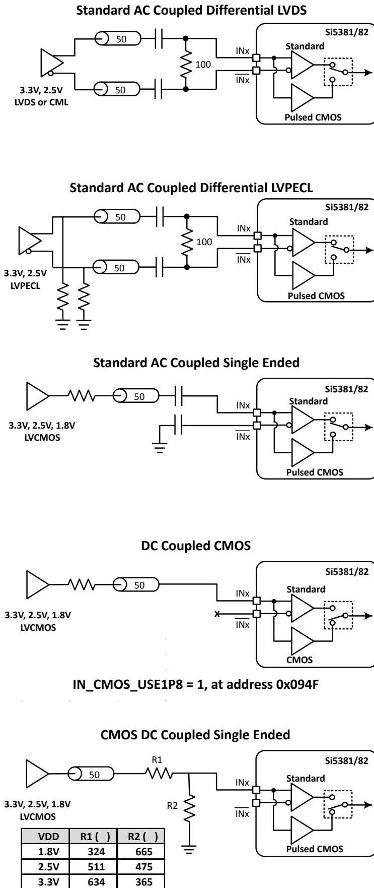
Figure 3.2. Input Termination for Standard and CMOS Inputs
