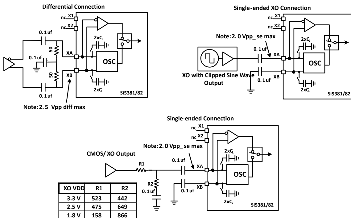
Figure 9.1. XAXB External XO Reference Clock Connection Options
