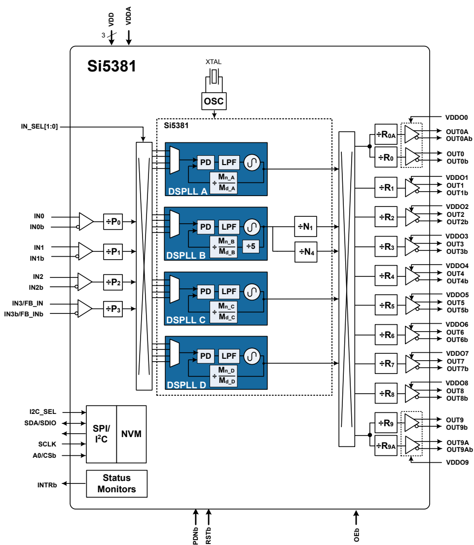
Figure 1.1. Si5381 Block Diagram
