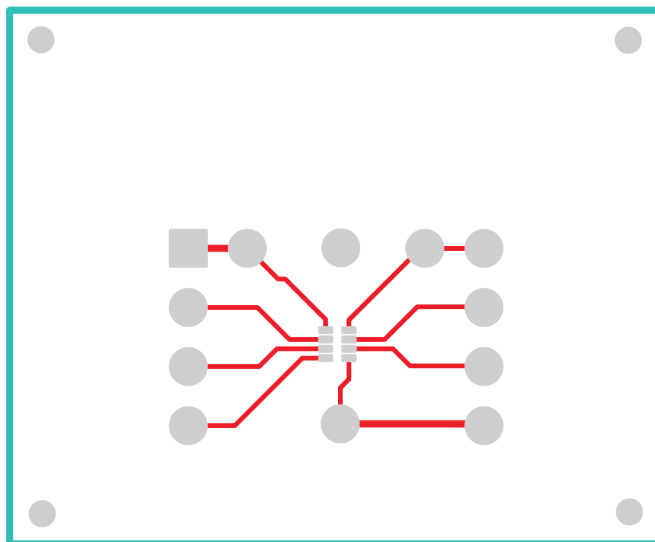
Figure 1. Top Layer
