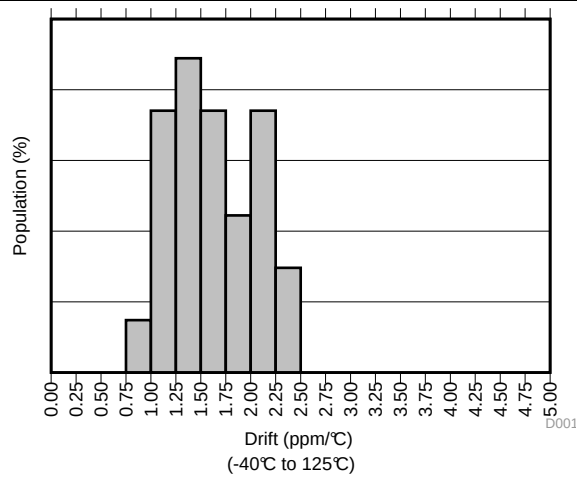
Figure 1. Temperature Drift
