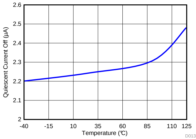
Figure 13. Quiescent Current Shutdown Mode
