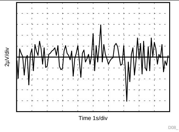
Figure 20. 0.1-Hz to 10-Hz Noise ( V_{REF} )
