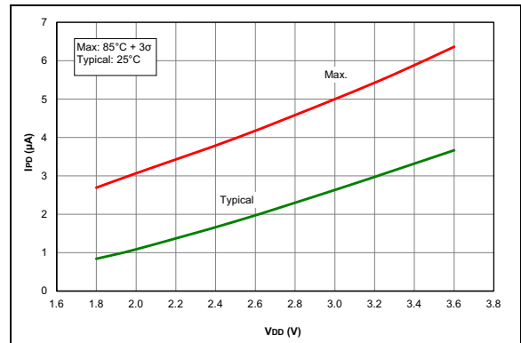
FIGURE 36-29: I_{PD} , Timer1 Oscillator, FOSC = 32 kHz, PIC16LF1614/8 Only.
