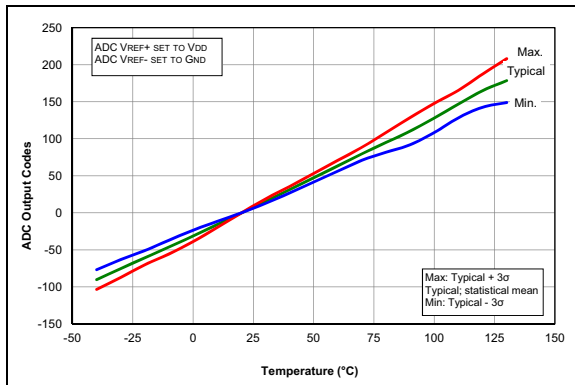
FIGURE 36-75: Temp. Indicator Slope Normalized to 20°C, High Range, V_{DD} = 3.0V , PIC16LF1614/8 Only.
