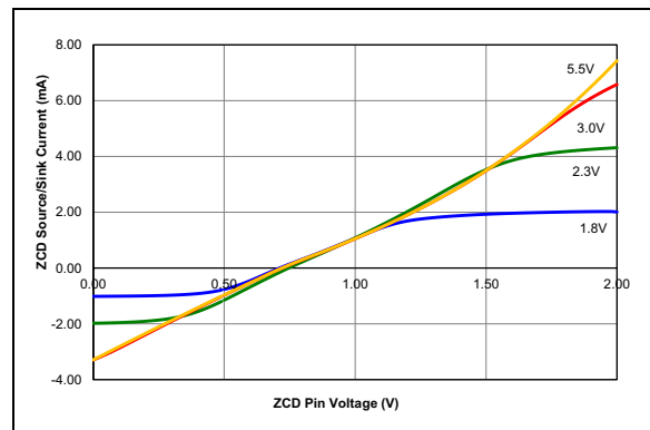
FIGURE 36-101: ZCD Pin Current over ZCD Pin Voltage, Typical Measured Values from -40^\circ\text{C} to 125^\circ\text{C} .
