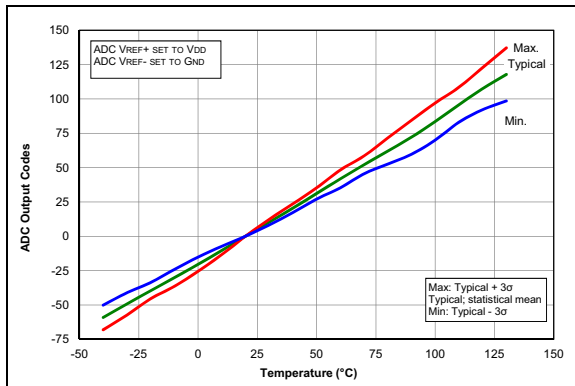
FIGURE 36-74: Temp. Indicator Slope Normalized to 20°C, High Range, V_{DD} = 5.5V , PIC16LF1614/8 Only.
