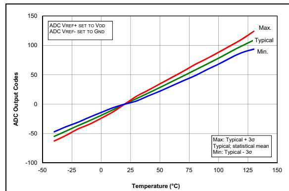
FIGURE 36-78: Temp. Indicator Slope Normalized to 20°C, Low Range, V_{DD} = 3.0V , PIC16LF1614/8 Only.
