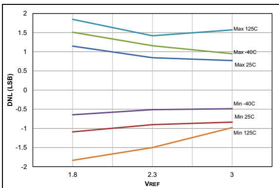
FIGURE 36-69: ADC 10-bit Mode, Single-Ended DNL, V_{DD} = 3.0V , T_{AD} = 1\ \mu\text{s} .
