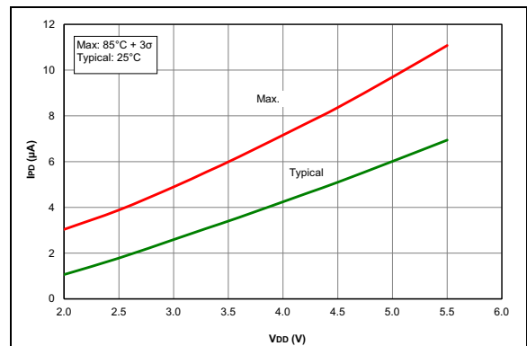
FIGURE 36-30: I_{PD} , Timer1 Oscillator, FOSC = 32 kHz, PIC16F1614/8 Only.
