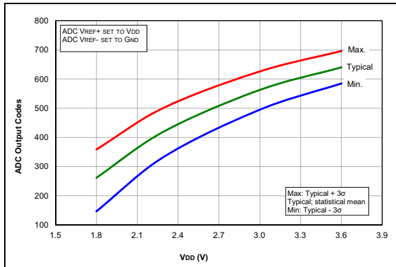
FIGURE 36-73: Temp. Indicator Initial Offset, Low Range, Temp. = 20°C, PIC16LF1614/8 Only.
