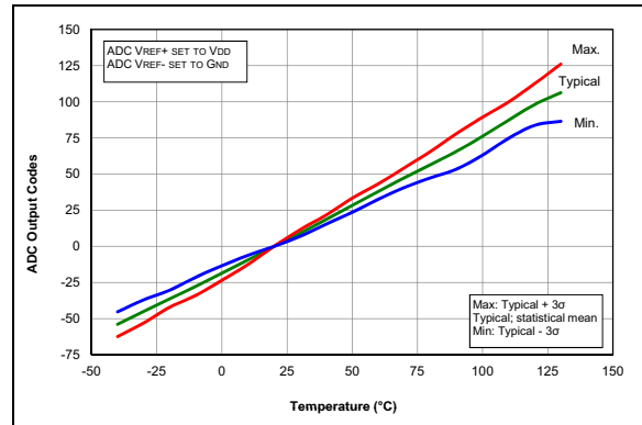
FIGURE 36-76: Temp. Indicator Slope Normalized to 20°C, Low Range, V_{DD} = 3.0V , PIC16LF1614/8 Only.
