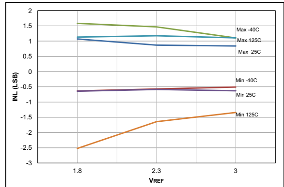
FIGURE 36-70: ADC 10-bit Mode, Single-Ended INL, V_{DD} = 3.0V , T_{AD} = 1\ \mu\text{s} .
