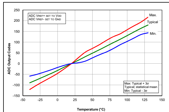
FIGURE 36-77: Temp. Indicator Slope Normalized to 20°C, Low Range, V_{DD} = 1.8V , PIC16LF1614/8 Only.
