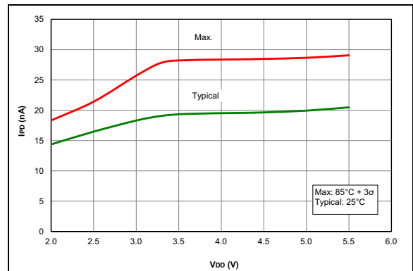
FIGURE 36-24: I_{PD} , Fixed Voltage Reference (FVR), PIC16F1614/8 Only.
