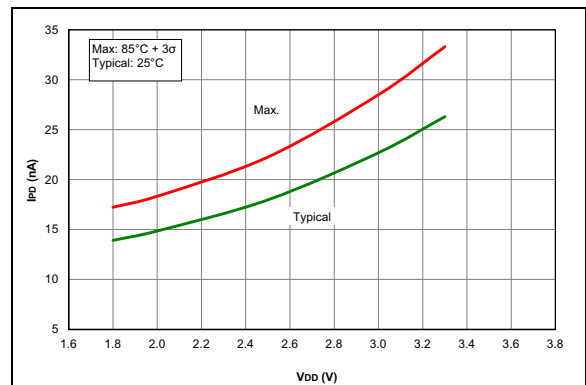
FIGURE 36-23: I_{PD} , Fixed Voltage Reference (FVR), PIC16LF1614/8 Only.
