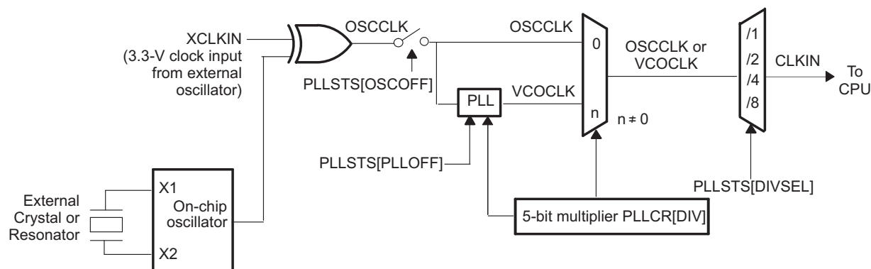
Figure 6-28. OSC and PLL Block Diagram
