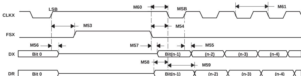
Figure 5-25. McBSP Timing as SPI Master or Slave: CLKSTP = 11b, CLKXP = 1
