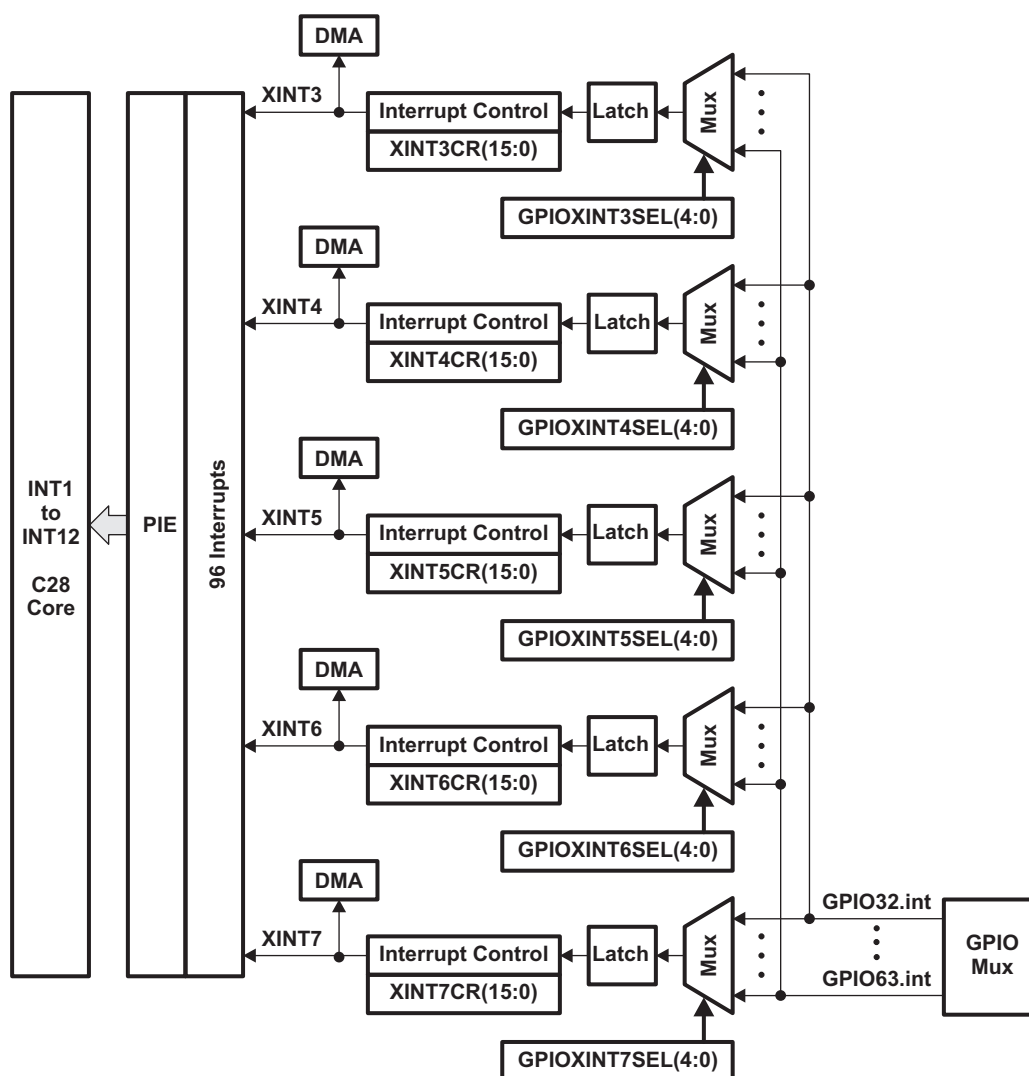
Figure 6-25. External Interrupts
