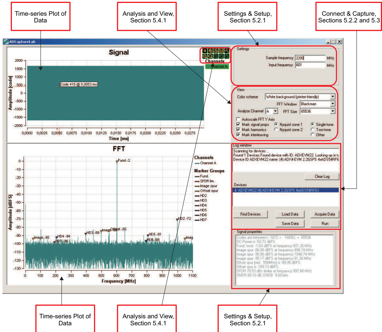
Figure 1. ADCapture Lab Main Window
