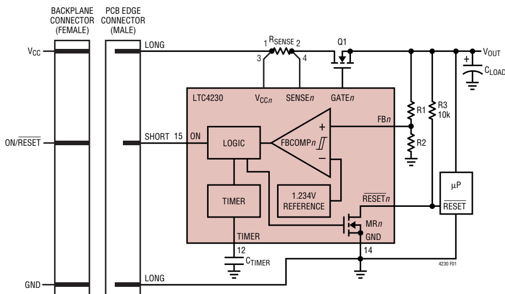
Figure 1. Supply Voltage Monitor Block Diagram
