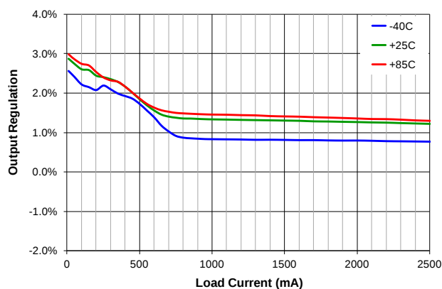
Figure 14. Output Regulation vs. Load Current and Temperature, V_{IN}=3.0\text{ V} , V_{OUT}=3.15\text{ V}
