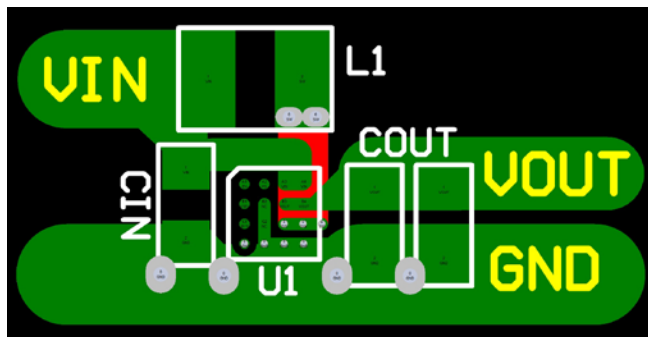
Figure 41. Layout Recommendation
