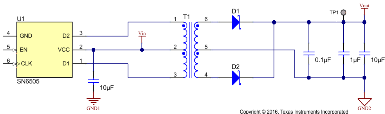
Figure 46. Unregulated Output for Low-Current Loads With Wide Supply Range
