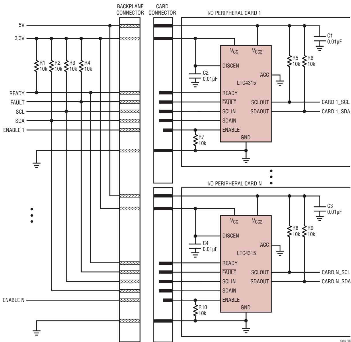
Figure 6. LTC4315 in an I 2 C Hot Swap Application with a Staggered Connector
