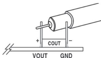
Figure 2. Measuring Output Voltage Ripple
