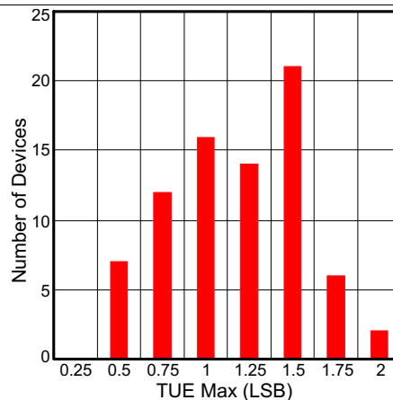
Figure 40. Total Unadjusted Error (TUE) Maximum
