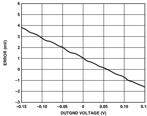
Figure 126. Typical DUTGND Transfer Function Voltage Error, Drive Low, V_{IL} = 0.0 \text{ V}
