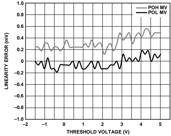
Figure 125. PPMU Go/No-Go Comparator Threshold INL
