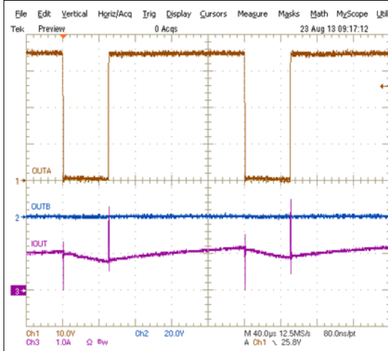
Figure 9. Forward Drive, Fast Decay
