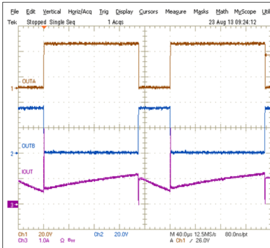
Figure 9. Forward Drive, Fast Decay
