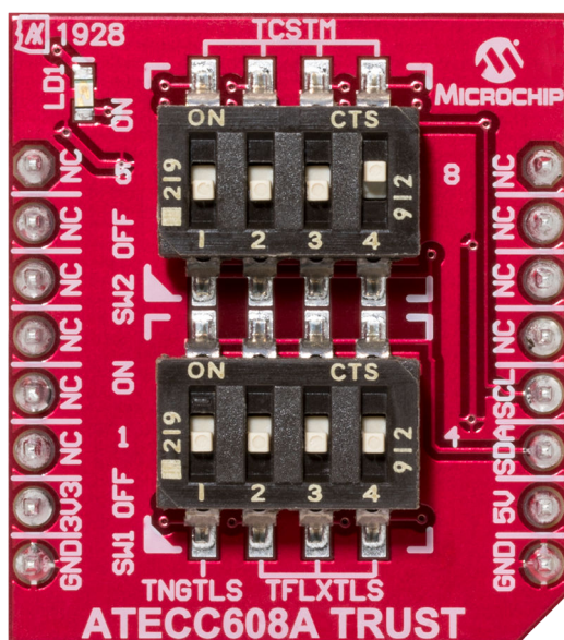
Figure 1. Front View
