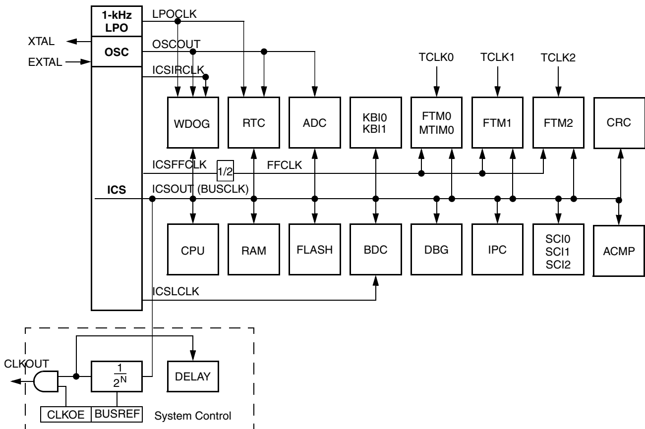
Figure 1-2. System clock distribution diagram
