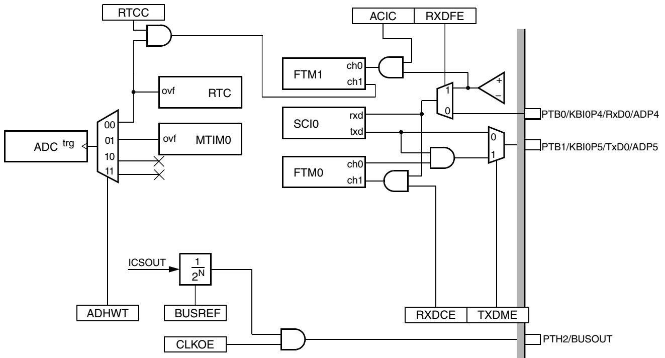
Figure 6-1. System interconnection diagram
