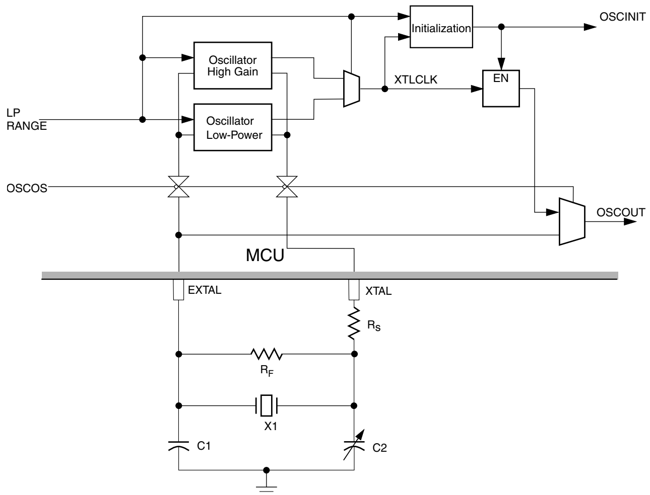
Figure 8-3. Oscillator module block diagram
