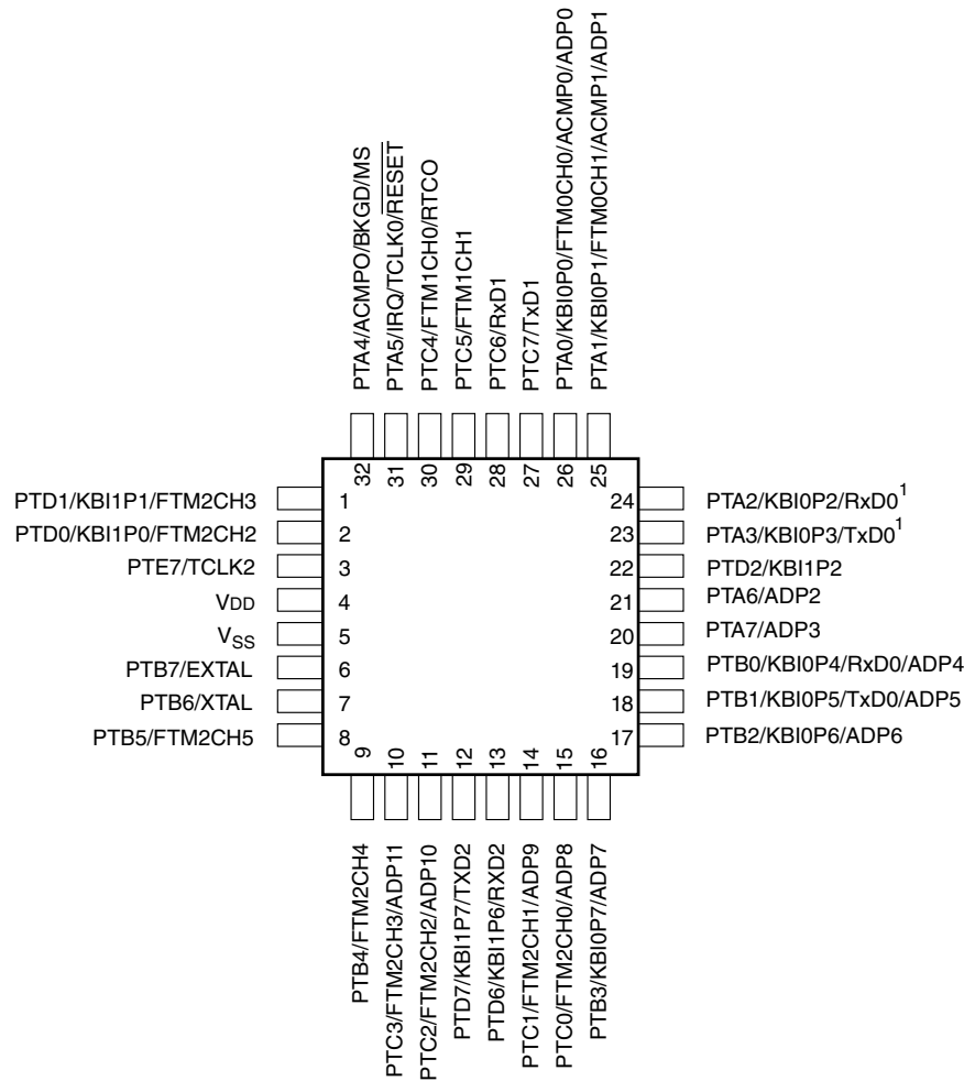
Figure 2-3. MC9S08PL60 32-pin LQFP package
