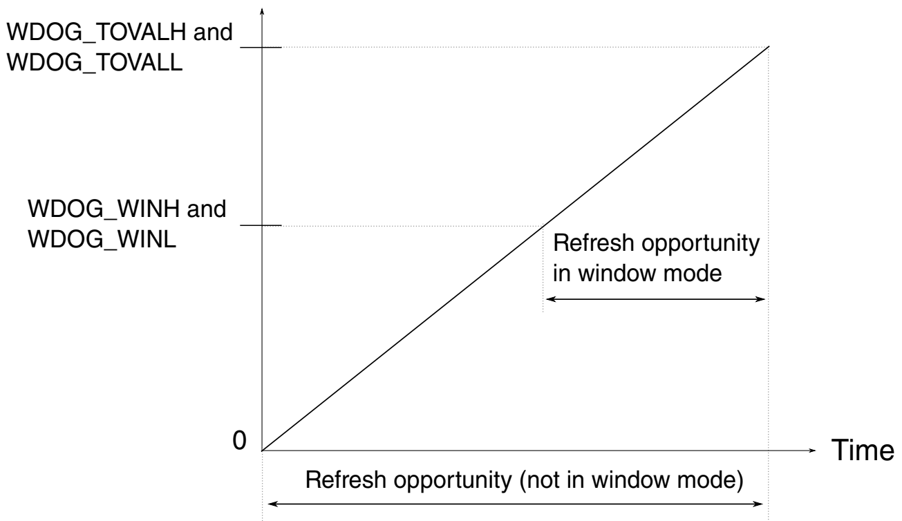
Figure 19-2. Refresh opportunity for the Watchdog counter
