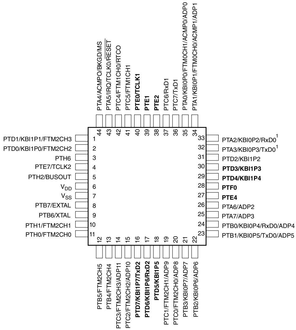
Figure 2-2. MC9S08PL60 44-pin LQFP package
