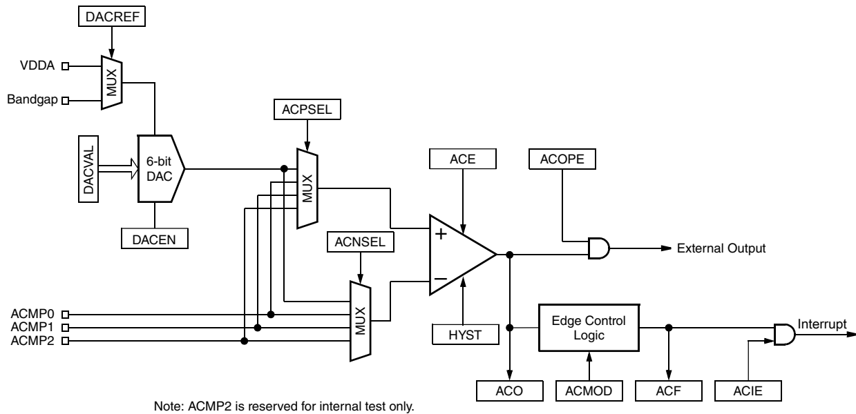
Figure 17-1. ACMP block diagram
