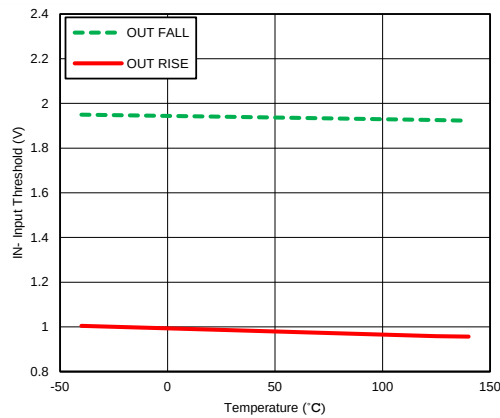
Figure 18. In- Input Threshold vs. Temperature
