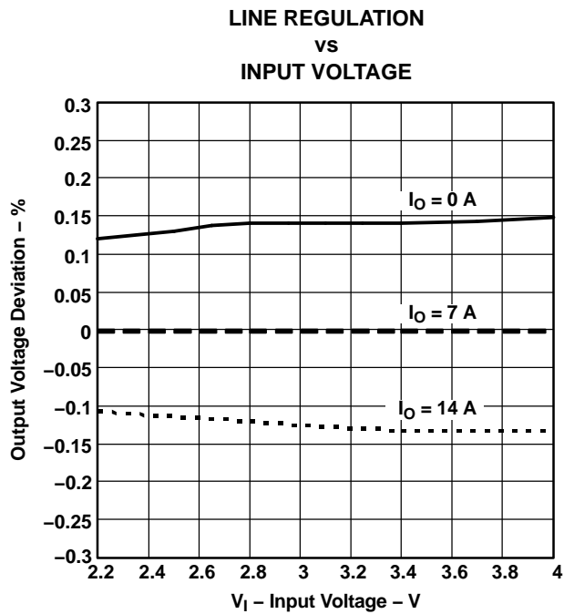
Figure 3. Line Regulation
