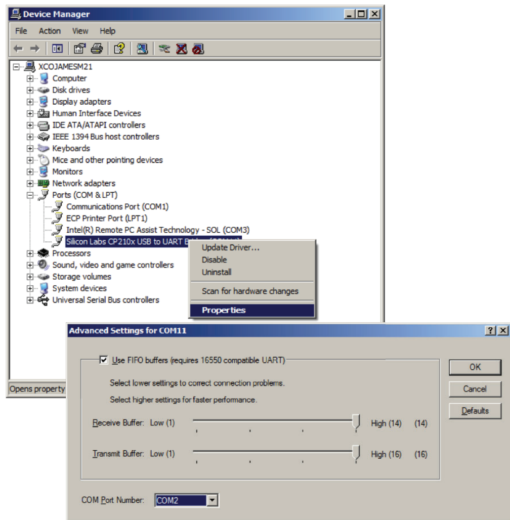
Figure 5: Port Selection on the Device Manager Screen
