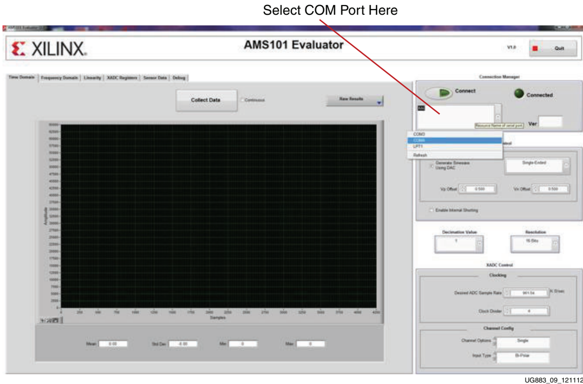
Figure 9: AMS101 Evaluator GUI
