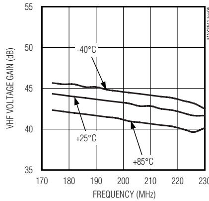
VHF VOLTAGE GAIN vs. FREQUENCY
