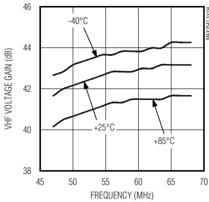
VHF VOLTAGE GAIN vs. FREQUENCY
