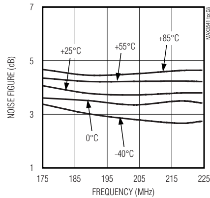
VHF NOISE FIGURE vs. FREQUENCY
