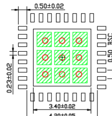
RECOMMENDED LAND PATTERN NOTE: 9, 10
