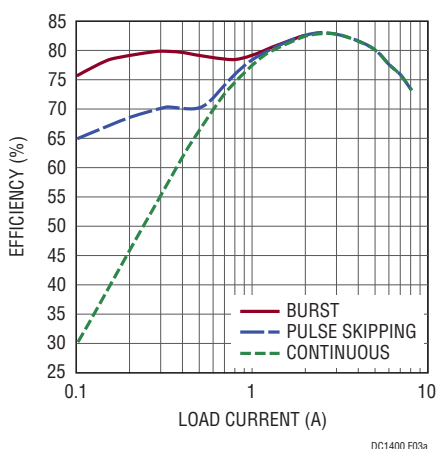
Efficiency vs Load Current with 3.3V_{IN} , 1.2V_{OUT}
