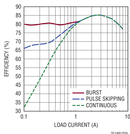
Efficiency vs Load Current with 3.3V_{IN} , 1.5V_{OUT}
