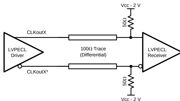
Figure 5. Differential LVPECL Operation, DC Coupling
