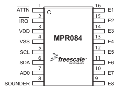
Figure 1. Pin Connections
