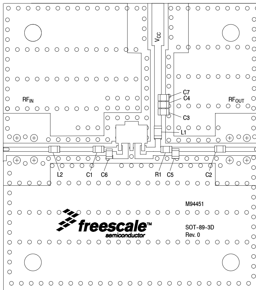
Figure 23. MMG30271BT1 Test Circuit Component Layout
