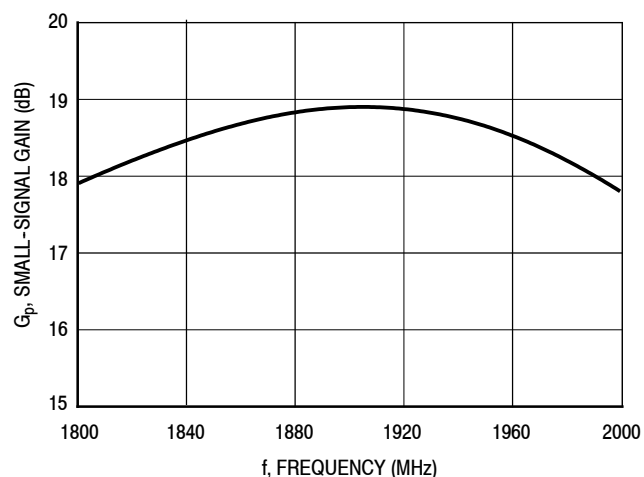
Figure 15. Small-Signal Gain (S21) versus Frequency
