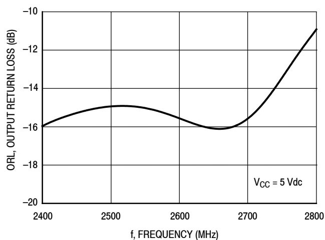
Figure 26. Output Return Loss (S22) versus Frequency
