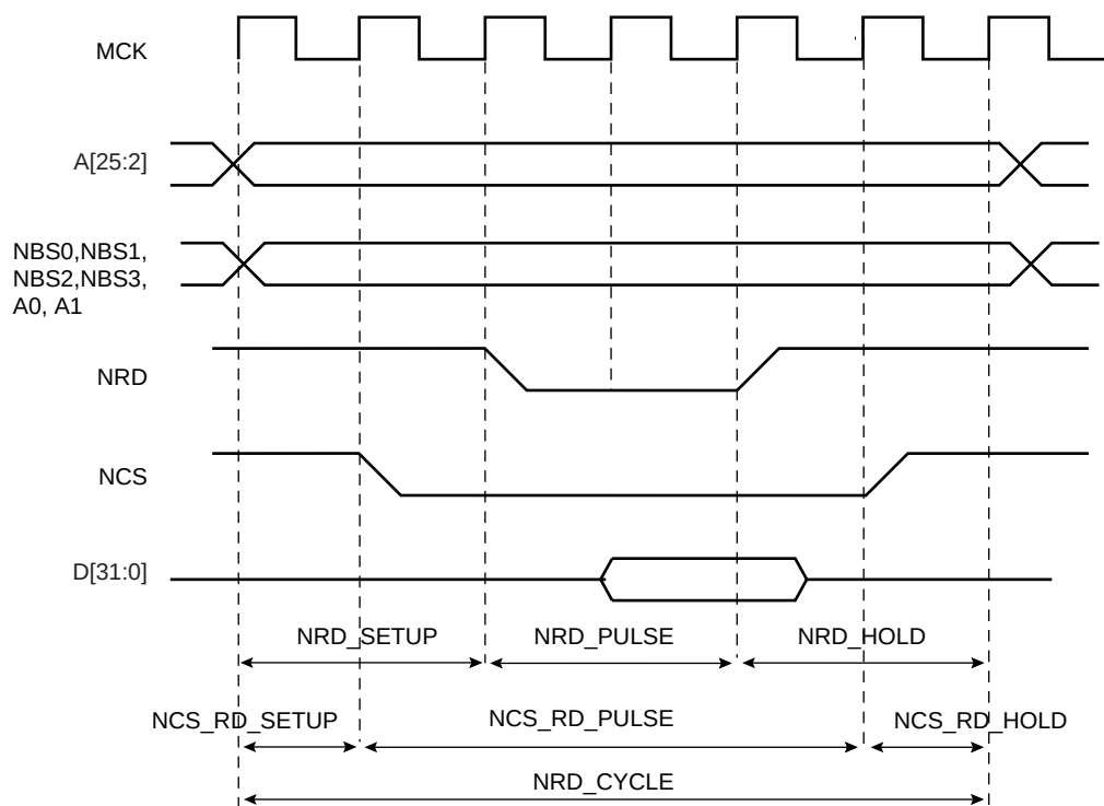
Figure 19-8. Standard Read Cycle
