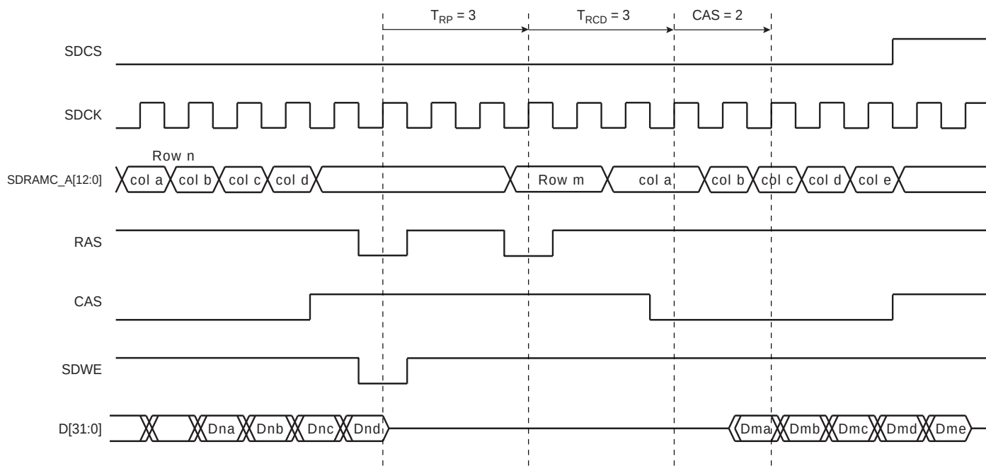
Figure 20-4. Read Burst with Boundary Row Access
