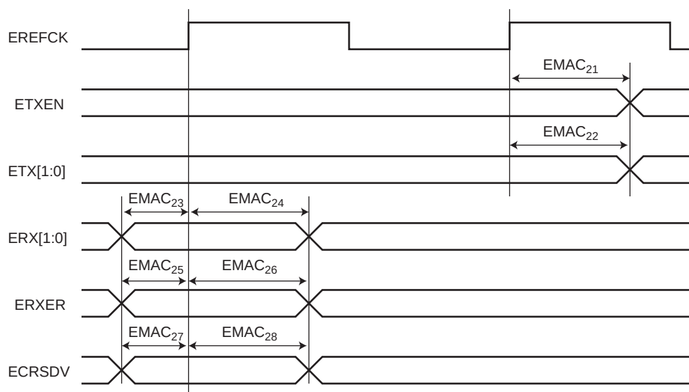
Figure 39-8. EMAC RMII Mode
