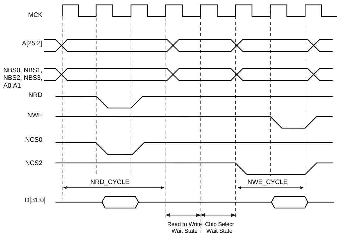
Figure 19-16. Chip Select Wait State between a Read Access on NCS0 and a Write Access on NCS2
