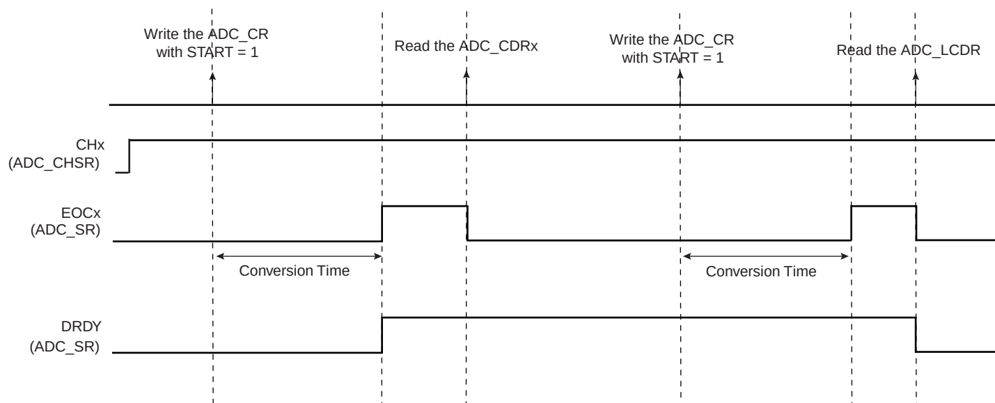
Figure 38-2. EOCx and DRDY Flag Behavior
