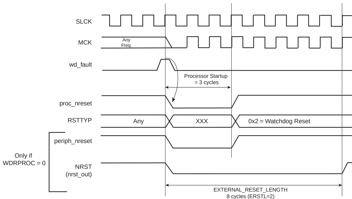
Figure 12-8. Watchdog Reset
