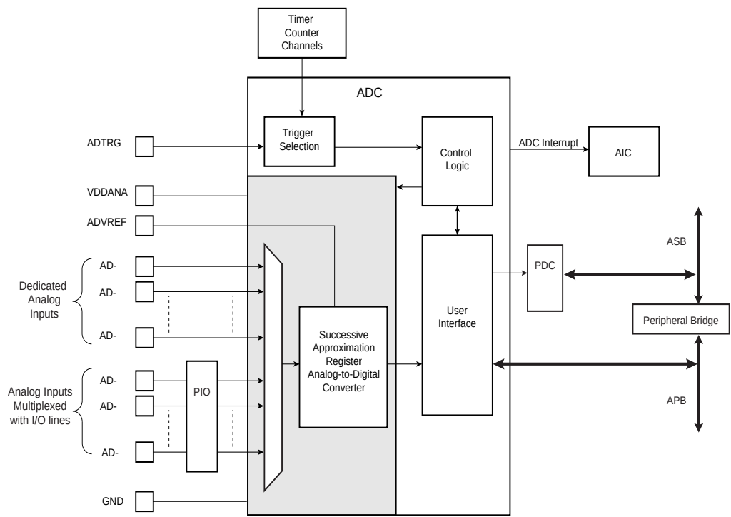
Figure 38-1. Analog-to-Digital Converter Block Diagram
