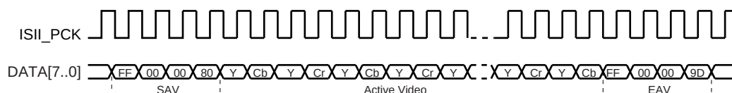
Figure 37-4. SAV and EAV Sequence Synchronization
