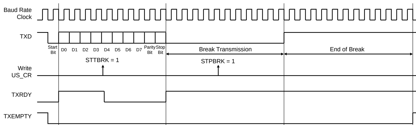
Figure 30-16. Break Transmission
