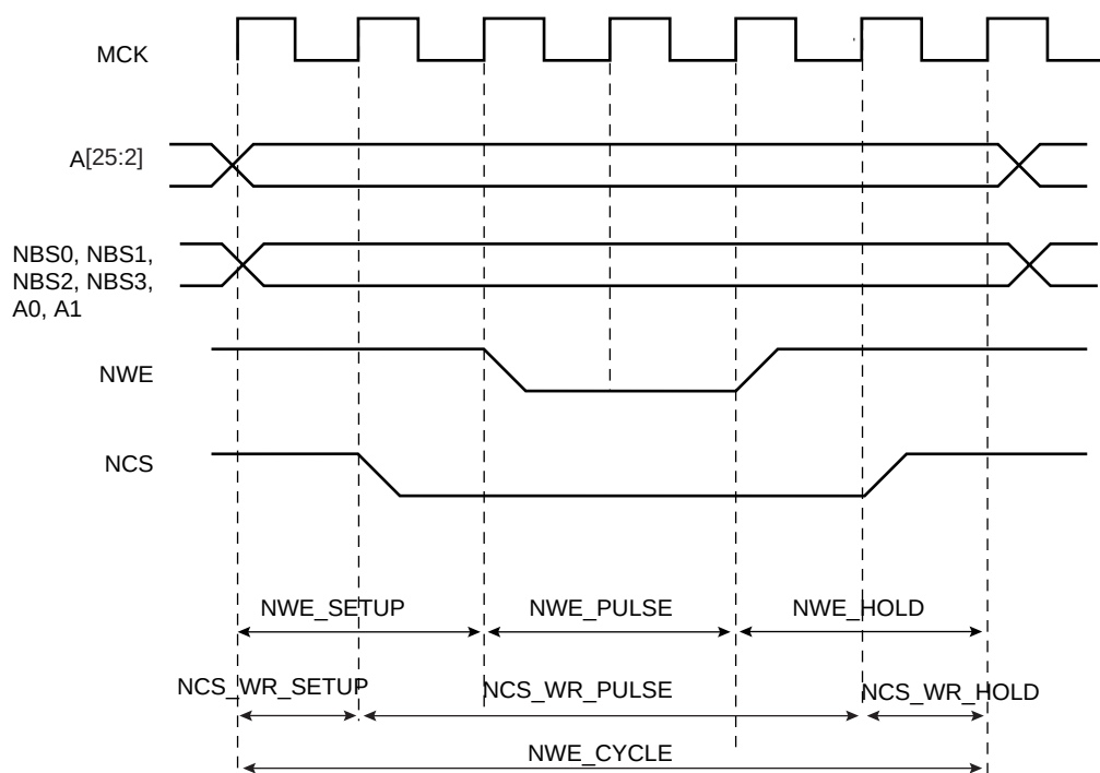
Figure 19-12. Write Cycle
