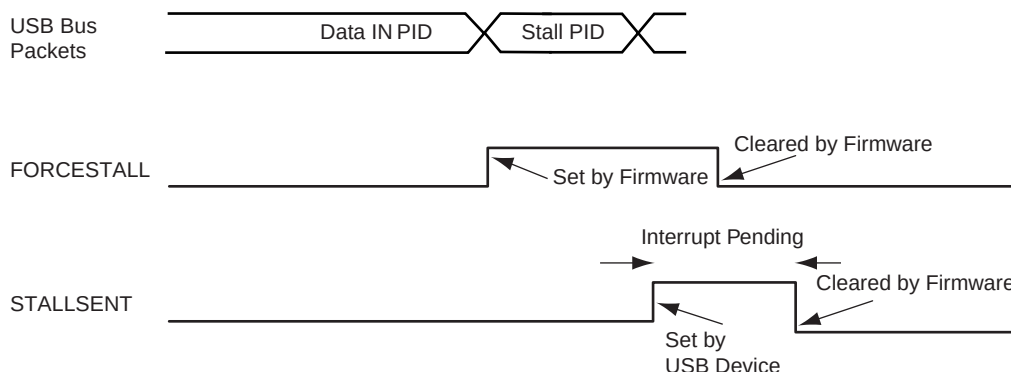
Figure 35-12. Stall Handshake (Data IN Transfer)
