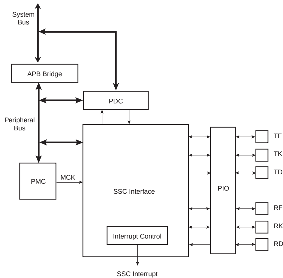
Figure 31-1. Block Diagram
