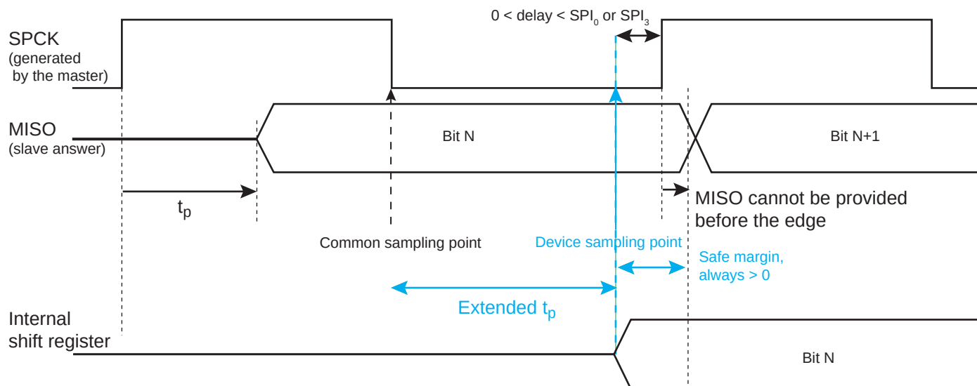
Figure 39-9. MISO Capture in Master Mode
