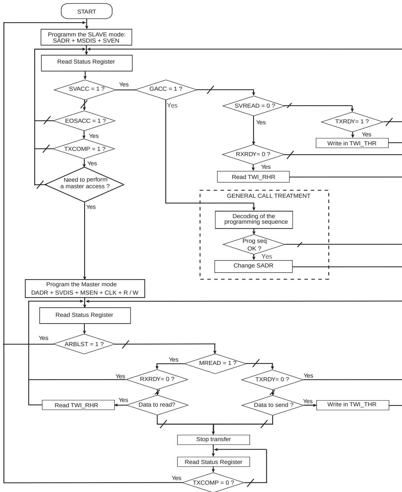
Figure 29-22. Multi-master Flowchart
