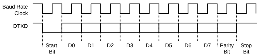
Figure 26-10. Character Transmission
