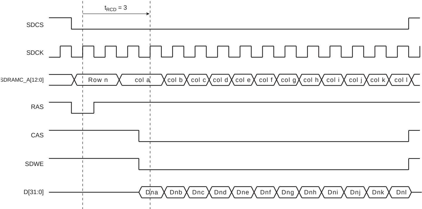
Figure 20-2. Write Burst, 32-bit SDRAM Access
