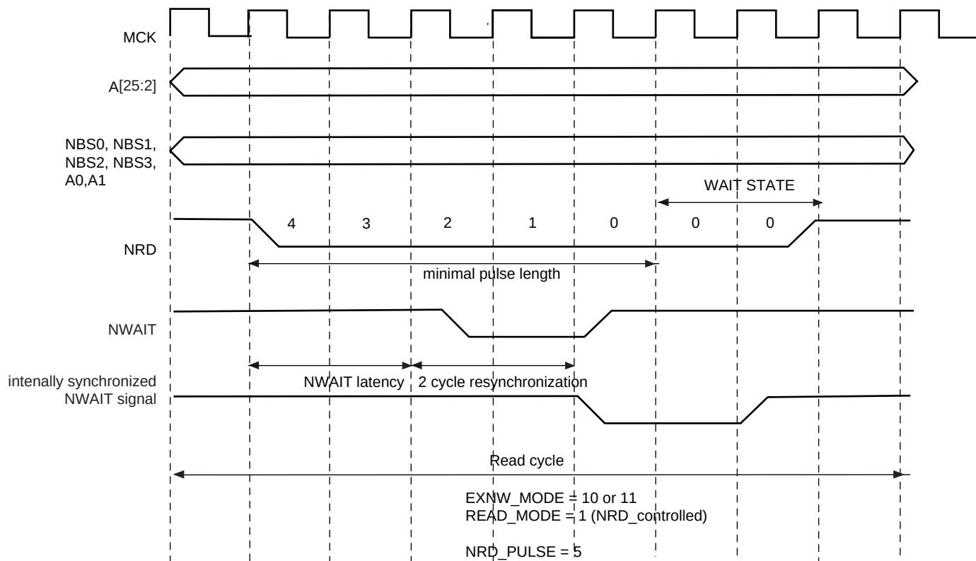
Figure 19-30. NWAIT Latency
