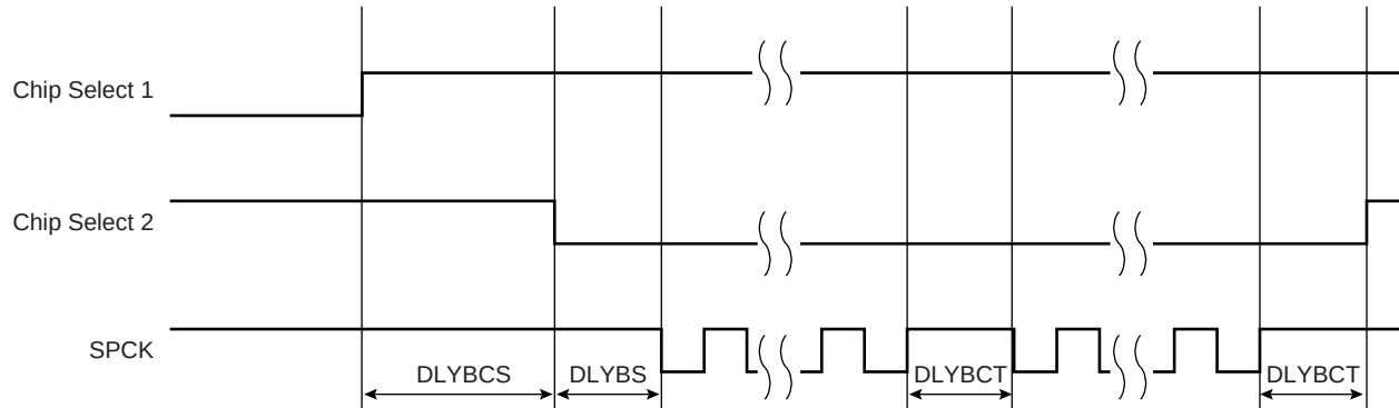
Figure 28-7. Programmable Delays
