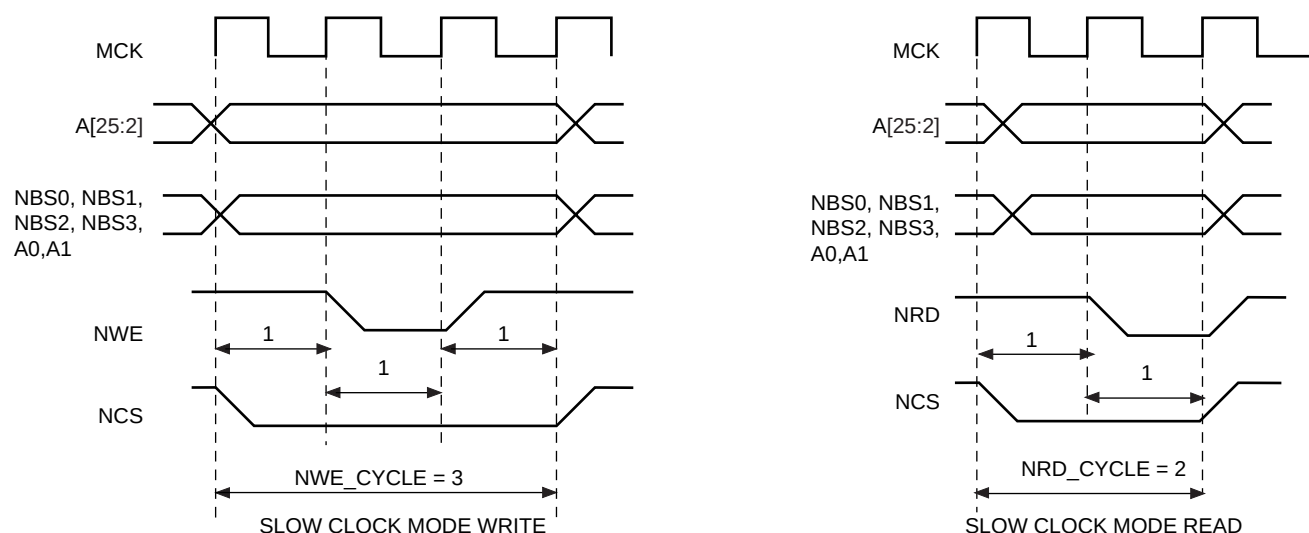
Figure 19-31. Read/Write Cycles in Slow Clock Mode
