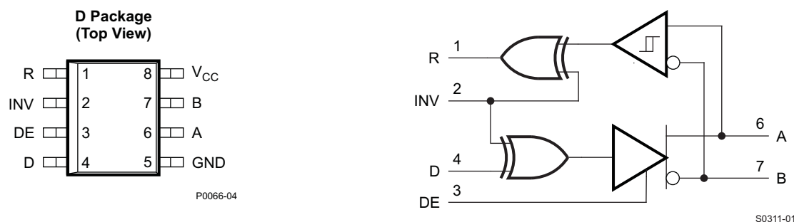
Figure 1. SN65HVD17xx With Inverting Feature to Correct for Miswired Cables
