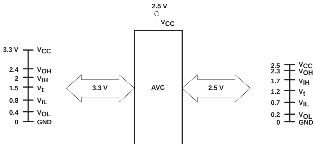
Figure 6. Device at 2.5-V V_{CC} With 3.3-V I/Os on One Side and 2.5-V I/Os on the Other, Showing Switching Levels
