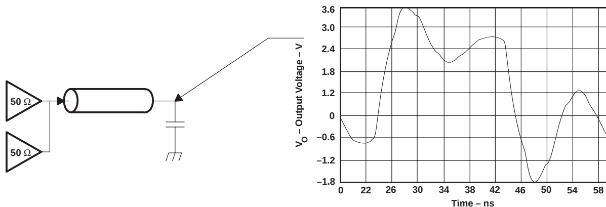
Figure 10. Two 50- \Omega Drivers In Parallel, Driving Transmission-Line Load and Waveform at the Load
