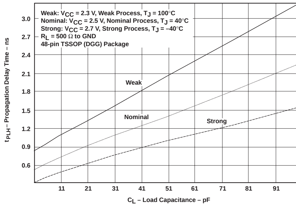
Figure 14. t_{PLH} vs Load Capacitance, One Output Switching
