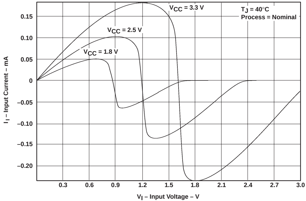
Figure 5. Bus Hold Across V_{CC}
