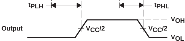
VOLTAGE WAVEFORMS PROPAGATION DELAY TIMES
