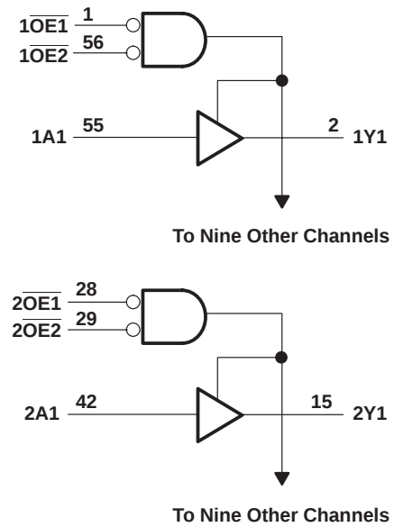
logic diagram (positive logic)
