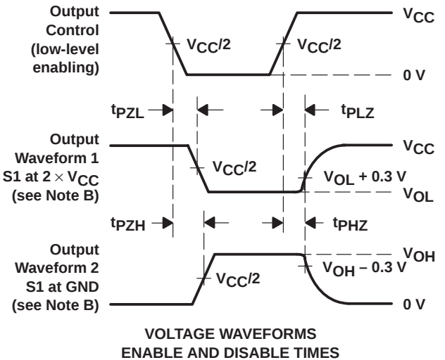
VOLTAGE WAVEFORMS PULSE DURATION
