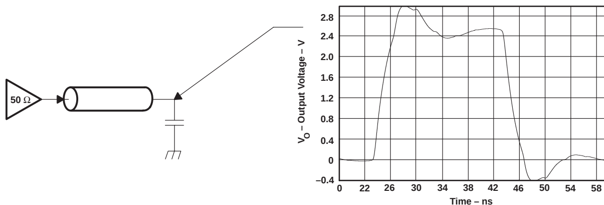
Figure 9. 50- \Omega Driver Driving Transmission-Line Load and Waveform at the Load
