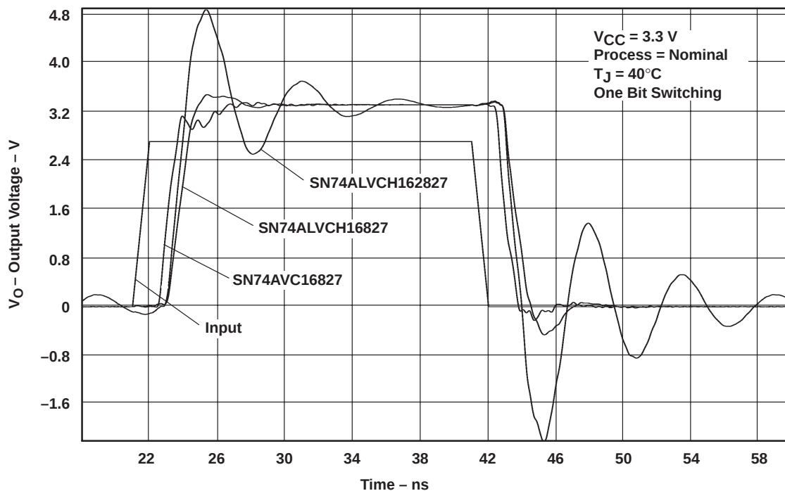
Figure 17. Outputs Driving a PC100 Load Network, V_{CC} = 3.3 V
