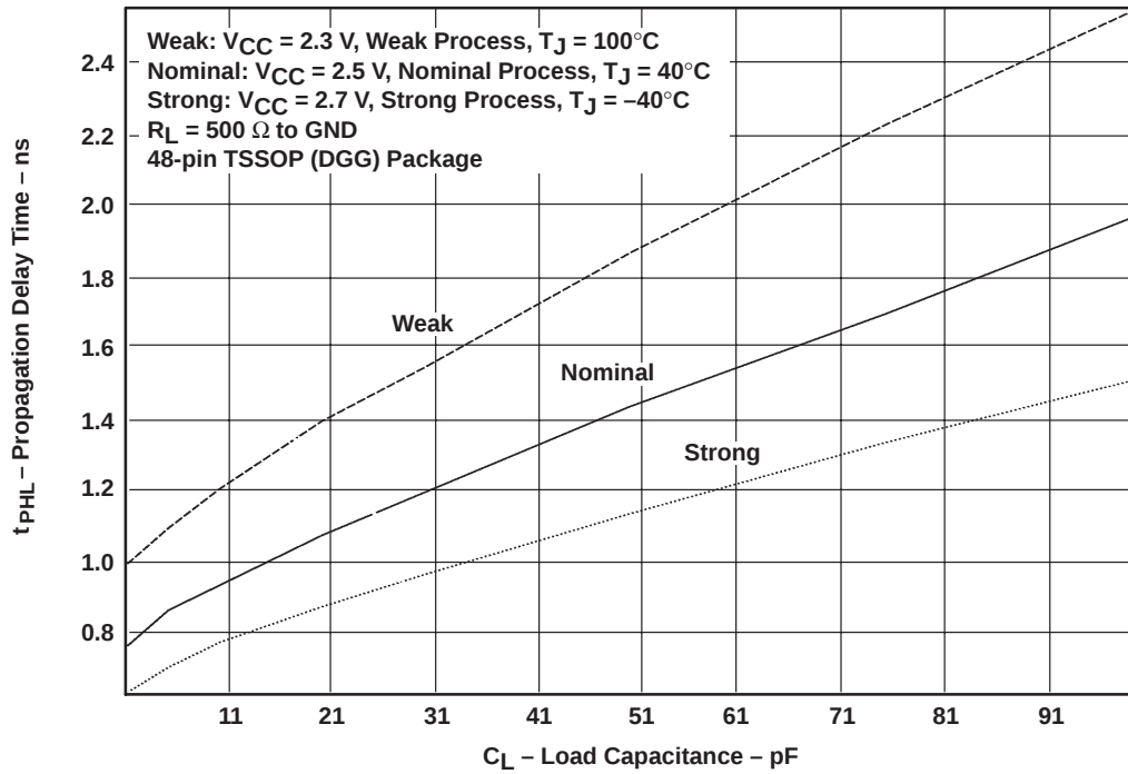
Figure 13. t_{PHL} vs Load Capacitance, One Output Switching
