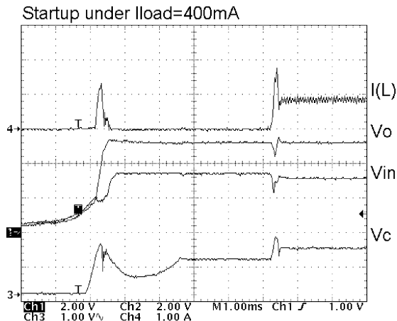
Figure 5. Startup Waveforms
