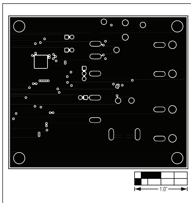
Figure 8. MAX97003 EV Kit PCB Layout—GND Layer 2
