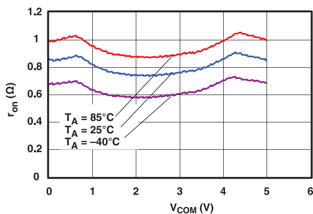
Figure 3. r_{on} vs V_{COM} ( V_+ = 5\text{ V} )
