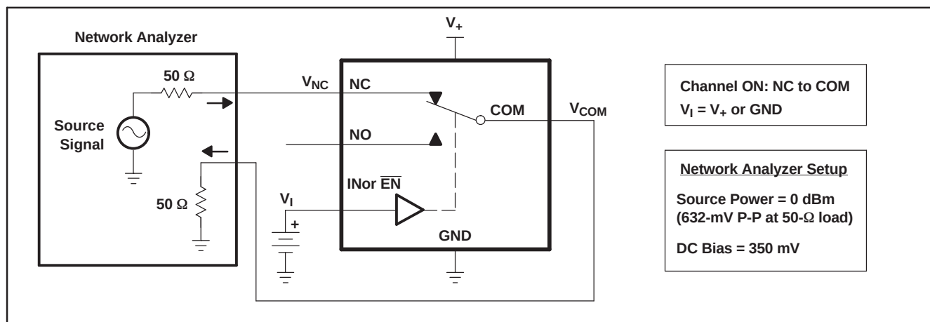
Figure 19. Bandwidth (BW)
