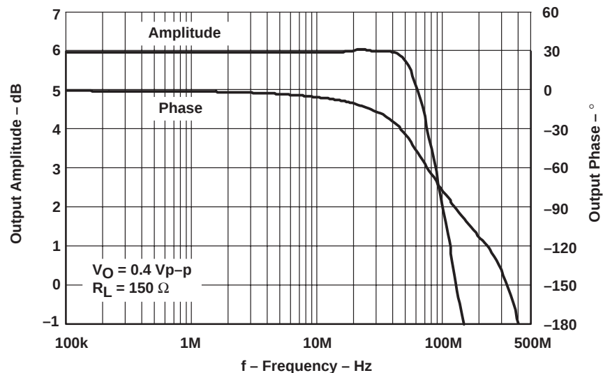
Figure 1–6. THS7001 EVM Preamplifier Response, V_{CC} = \pm 5 V
