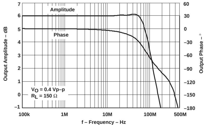
Figure 1–5. THS7001 EVM Preamplifier Response, V_{CC} = \pm 15 V
