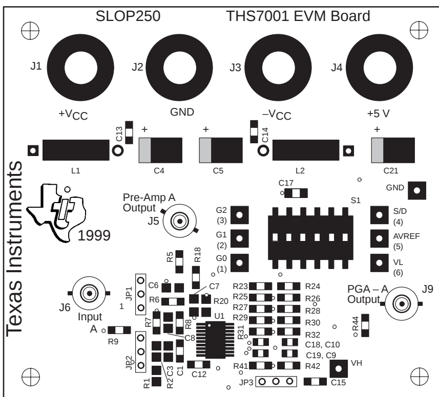
Figure 1–1. THS7001 Evaluation Module
