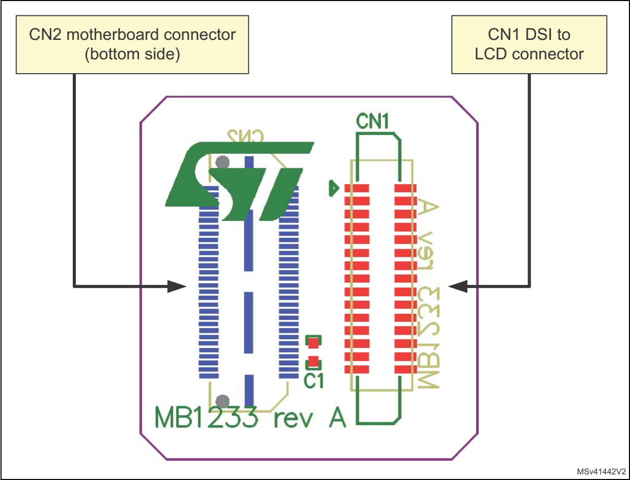
Figure 3. Board layout
