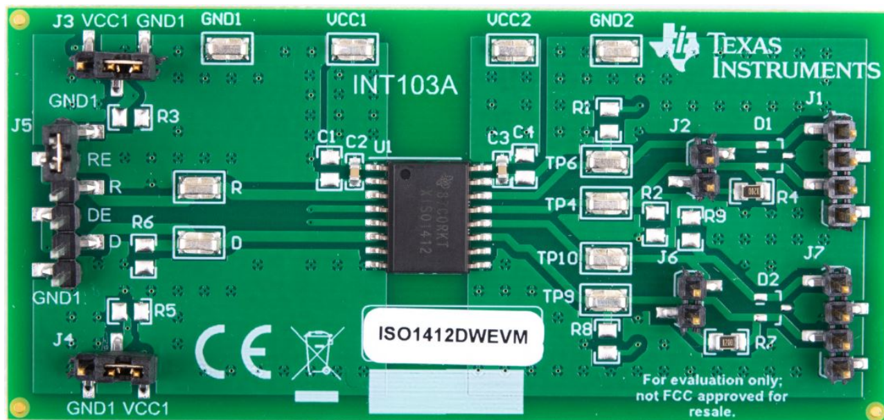
Figure 3. Board Layout
