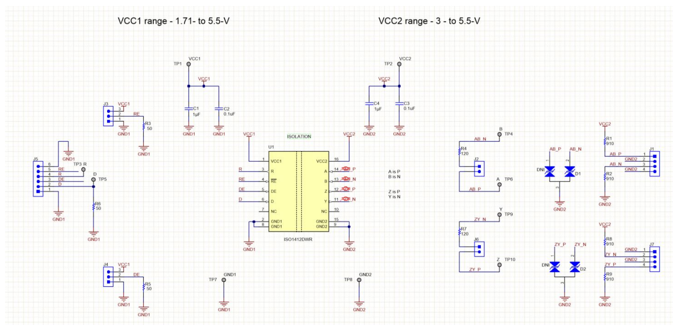
Figure 5. ISO1412DWEVM Schematic
