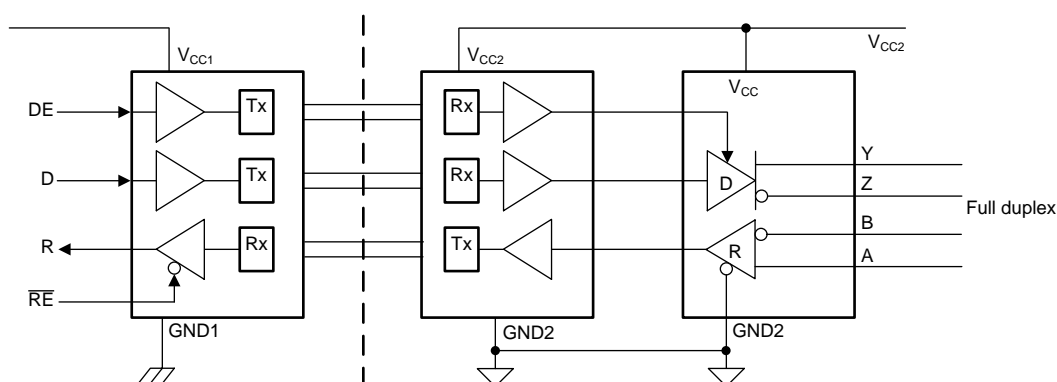
Figure 1. ISO1412 Functional Block Diagram
