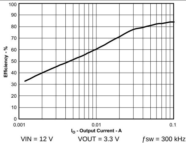
Figure 55. Light-Load Efficiency
