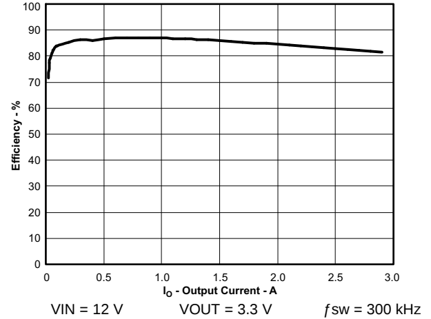
Figure 54. Efficiency vs Load Current
