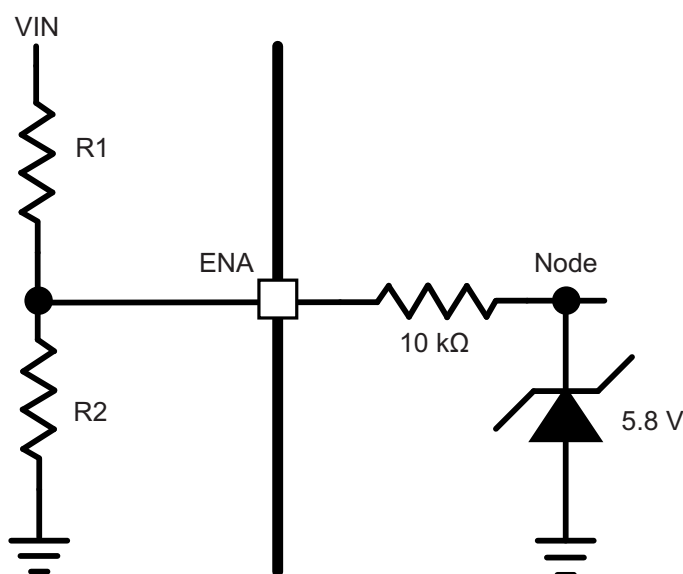
Figure 25. Node Voltage
