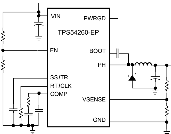
Simplified Schematic
