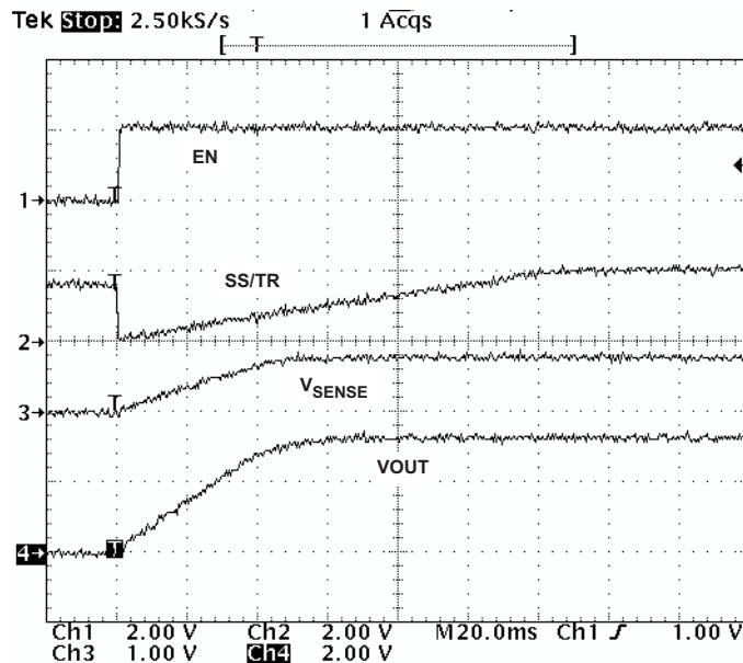
Figure 26. Operation of SS/TR Pin When Starting
