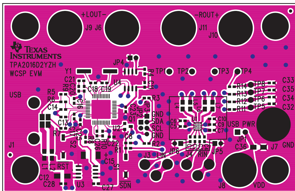
Figure 7. TPA2016D2EVM – Top Layer
