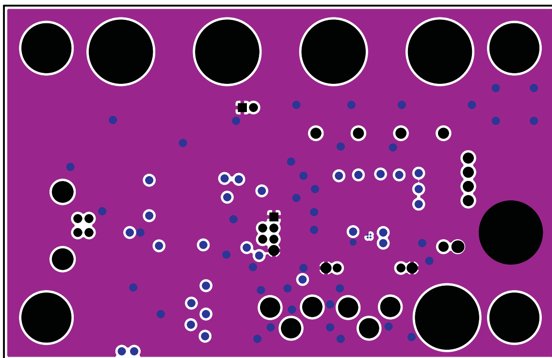
Figure 8. TPA2016D2EVM – Layer 2
