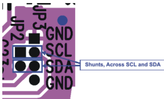
Figure 1. Place Shunts Horizontally Across SCL and SDA
