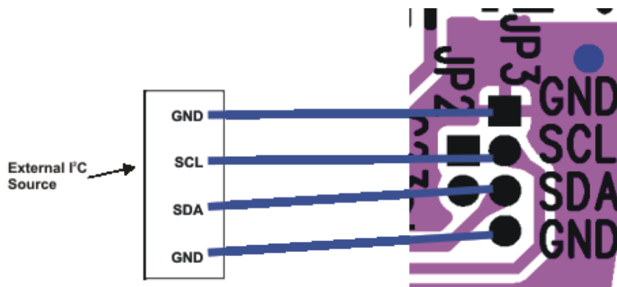
Figure 5. Connect I 2 C Controls to JP3
