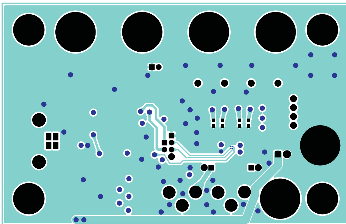
Figure 10. TPA2016D2EVM – Bottom Layer
