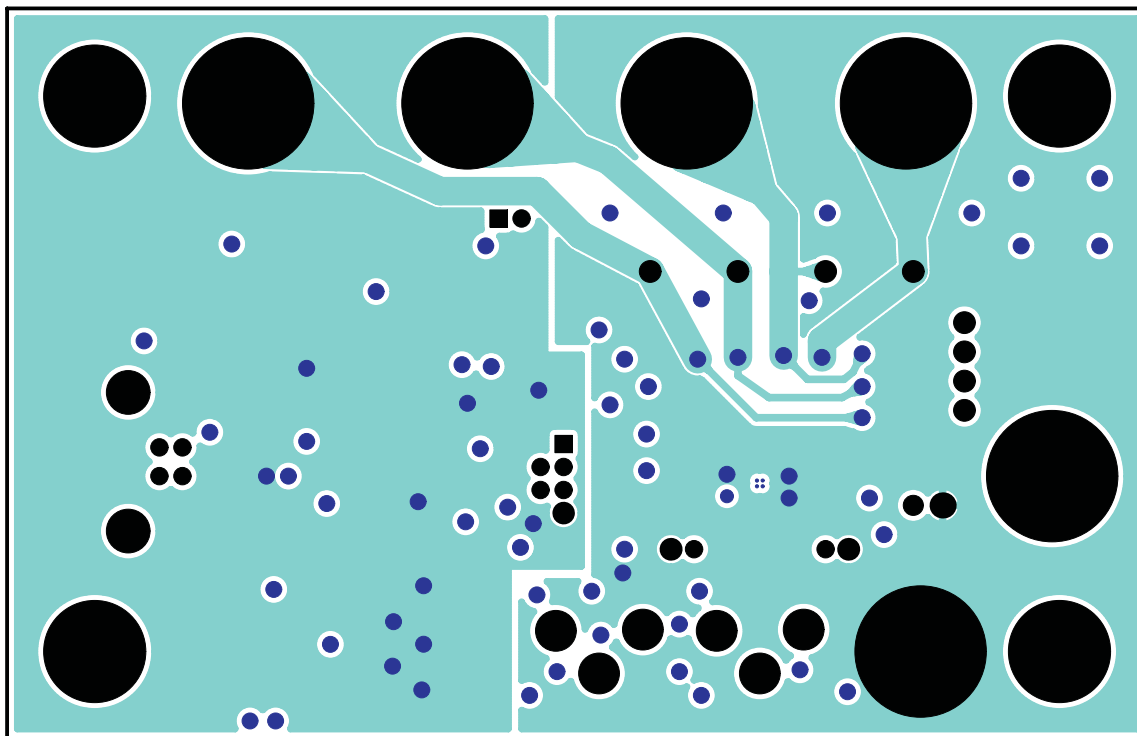
Figure 9. TPA2016D2EVM – Layer 3
