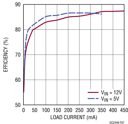
Figure 7. DC2449A-B Efficiency
