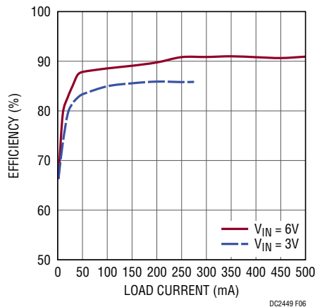
Figure 6. DC2449A-A Efficiency
