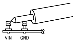
Figure 3. Measuring Input or Output Ripple
