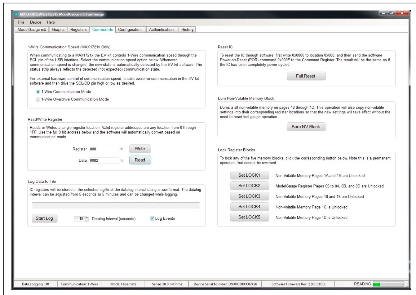
Figure 11. Commands Tab
