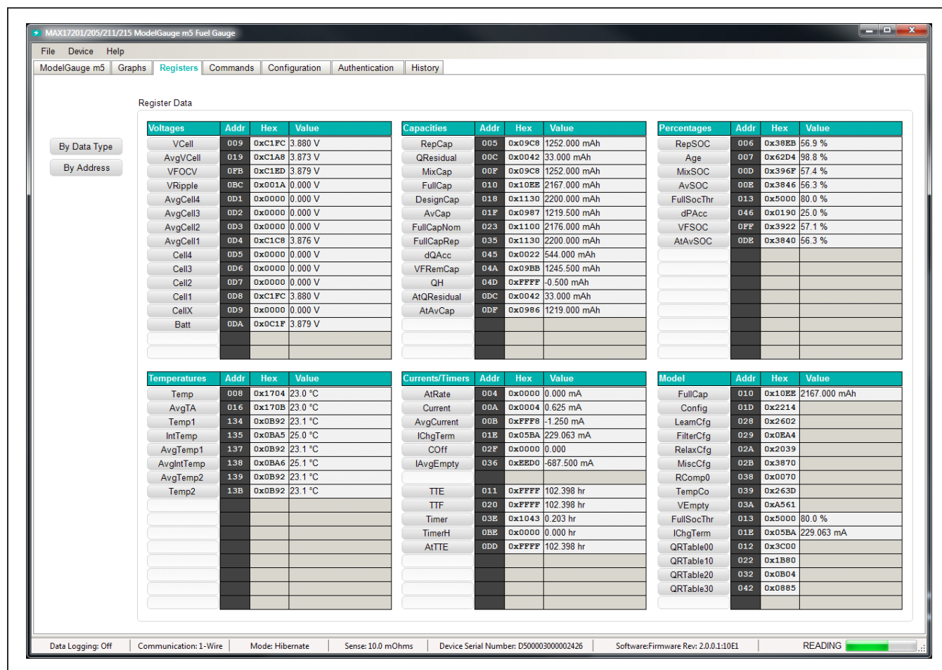
Figure 9. Registers Tab
