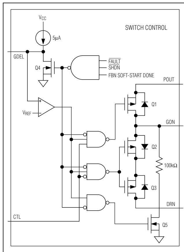
Figure 6. High-Voltage Switch Control Block Diagram
