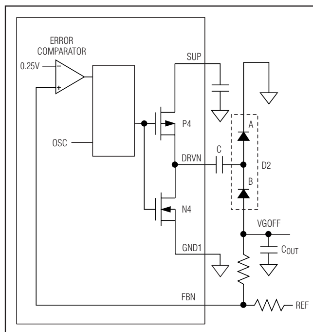
Figure 5. Negative Charge-Pump Regulator Block Diagram
