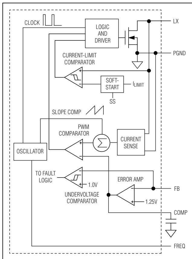
Figure 3. Step-Up Regulator PWM Control Block Diagram
