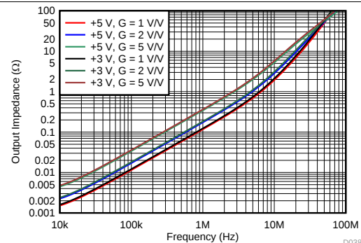
Figure 38. Closed-Loop Output Impedance vs Frequency
