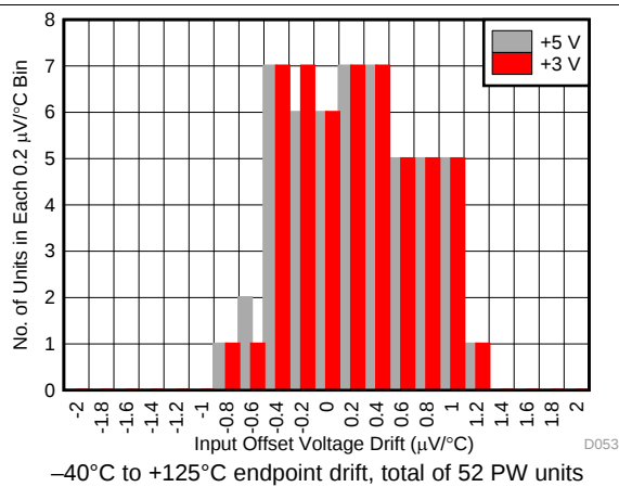
Figure 53. Input Offset Voltage Drift Histogram
