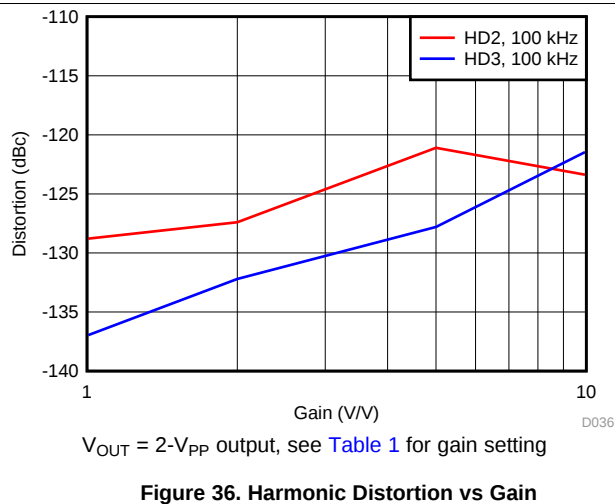
Figure 36. Harmonic Distortion vs Gain
