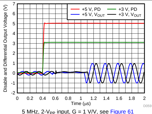
Figure 59. \overline{PD} Turn-On Waveform
