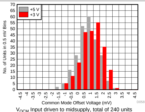
Figure 58. Common-Mode Output Offset from Driven V_{OCM} Histogram
