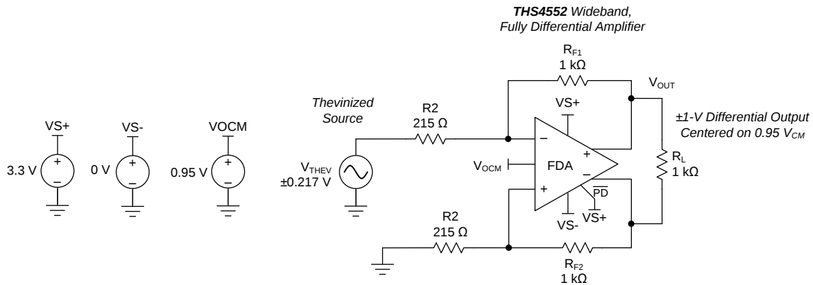
Figure 72. Input V_{ICM} Analysis Circuit From the Design of Figure 96
