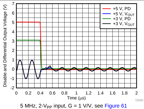
Figure 60. \overline{PD} Turn-Off Waveform
