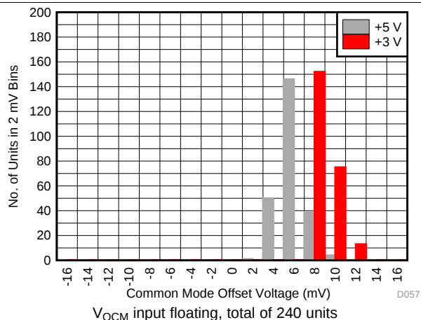
Figure 57. Common-Mode Output Offset from V_{S+} / 2 Default Value Histogram
