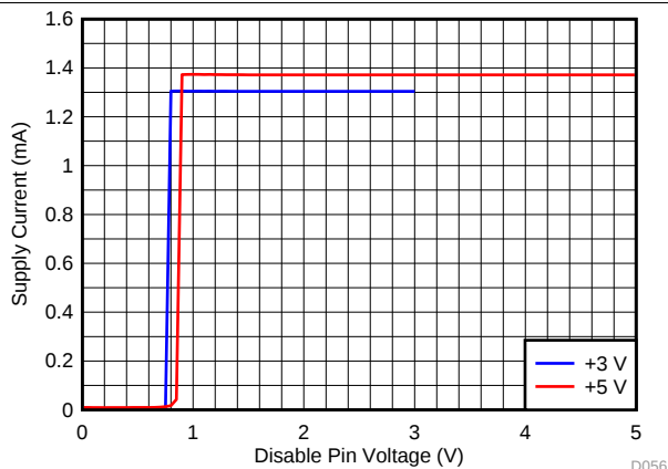
Figure 56. Supply Current vs \overline{PD} Voltage
