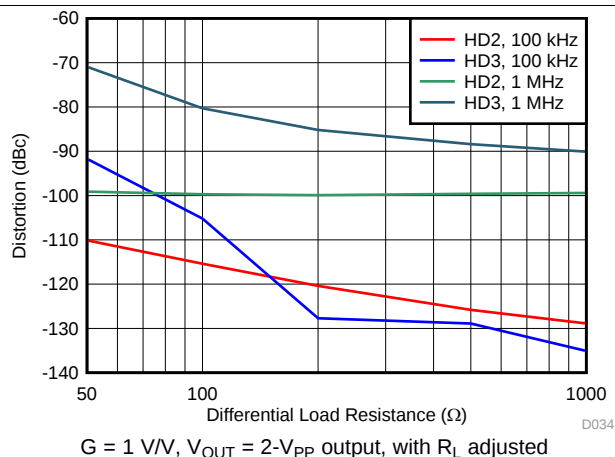
Figure 34. Harmonic Distortion vs R_L
