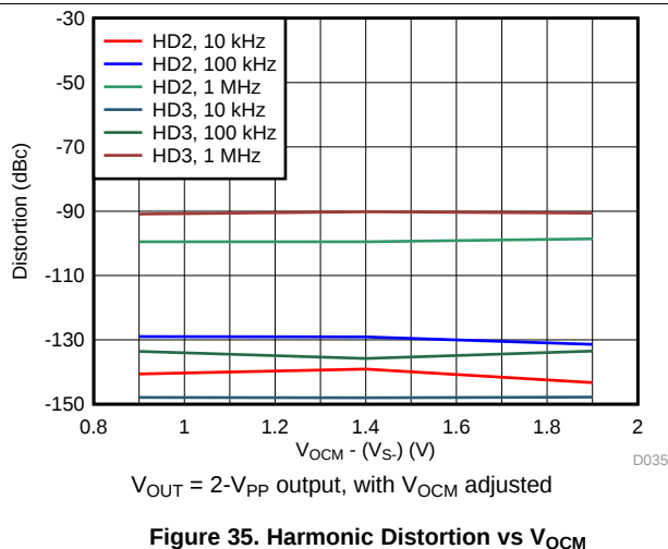
Figure 35. Harmonic Distortion vs V_{OCM}
