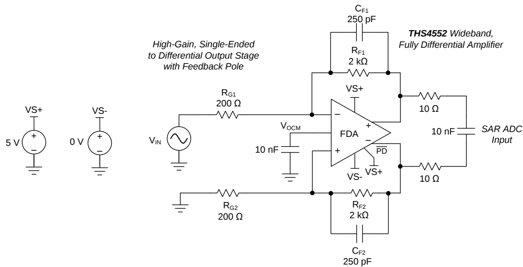
Figure 86. Single-Ended to Differential Stage with a Feedback Pole
