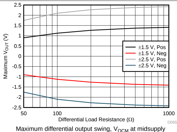
Figure 55. \pm Maximum V_{OUT} vs Differential Load Resistance
