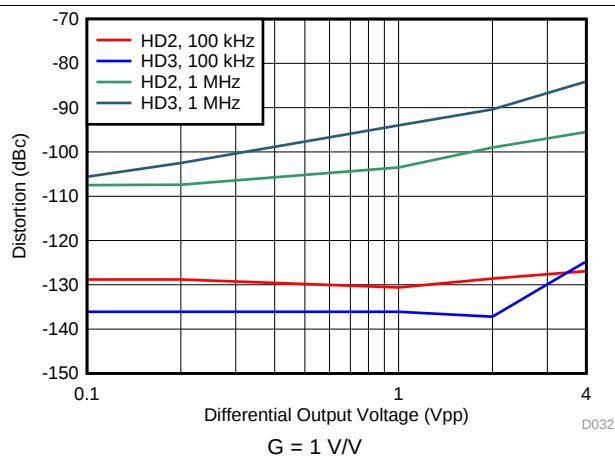
Figure 32. Harmonic Distortion vs Output Swing
