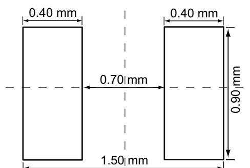
Figure 11. Alternative footprint, dimensions in mm
